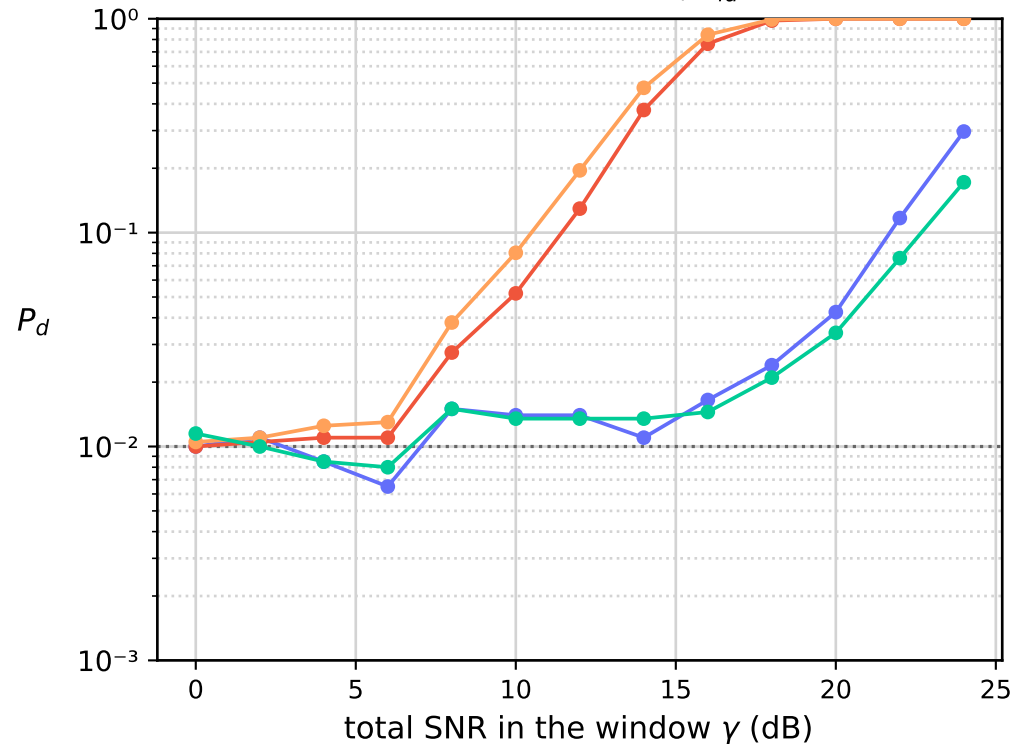
Channelized radiometer, P_{fa} = 10^{-2}
