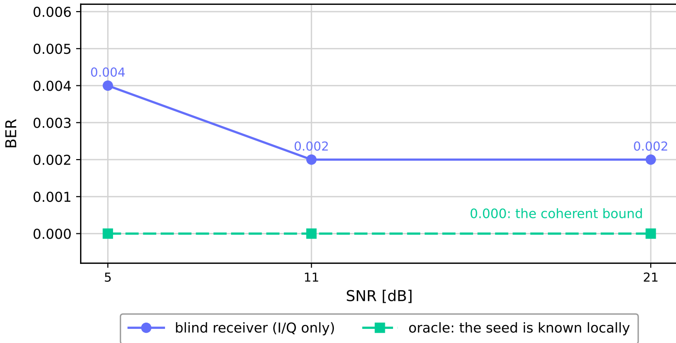
The price of blindness
