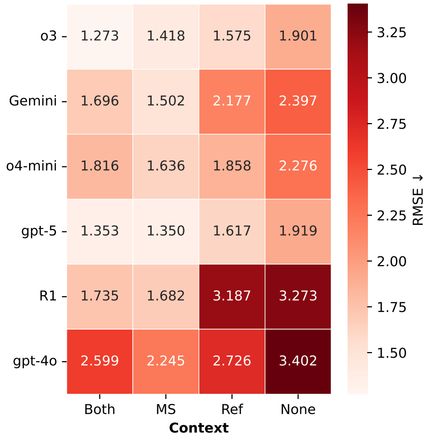
RMSE ↓
