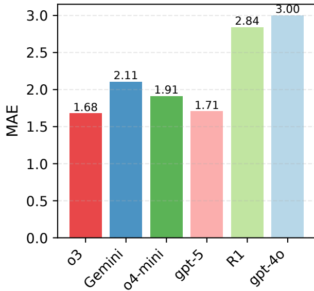
MAE ( \downarrow )
