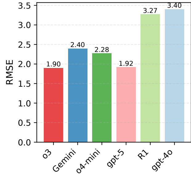
RMSE ( \downarrow )
