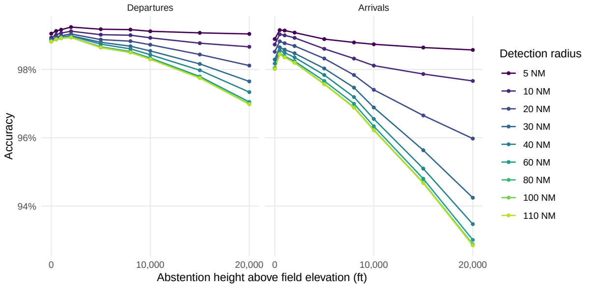
Figure 2: Accuracy against abstention height, same axes. This is the figure the coverage plot hides. Accuracy peaks close to the ground – at 40 NM, departures at 2,000 ft and arrivals at 500 ft – and every foot admitted above that is bought with correctness: -1.00 pp for departures by 15,000 ft, -3.47 pp for arrivals. The radius, which barely touches coverage above 40 NM, spreads accuracy at 15,000 ft by +1.32 pp for departures and +3.97 pp for arrivals.
