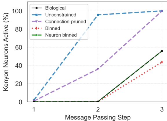
Kenyon Cell Types Activation
