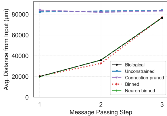
Activation Propagation Distance
