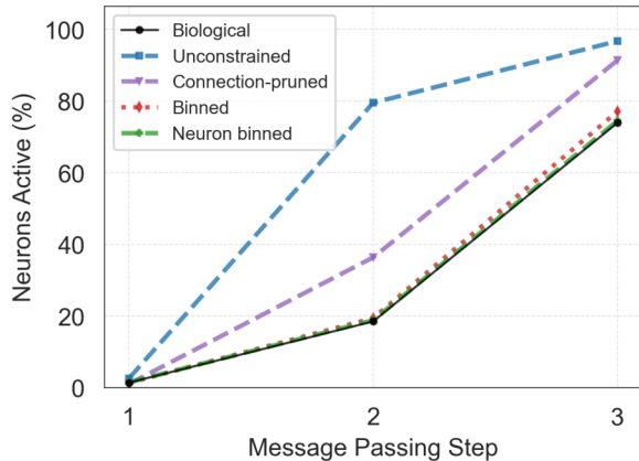
Neural Activation
