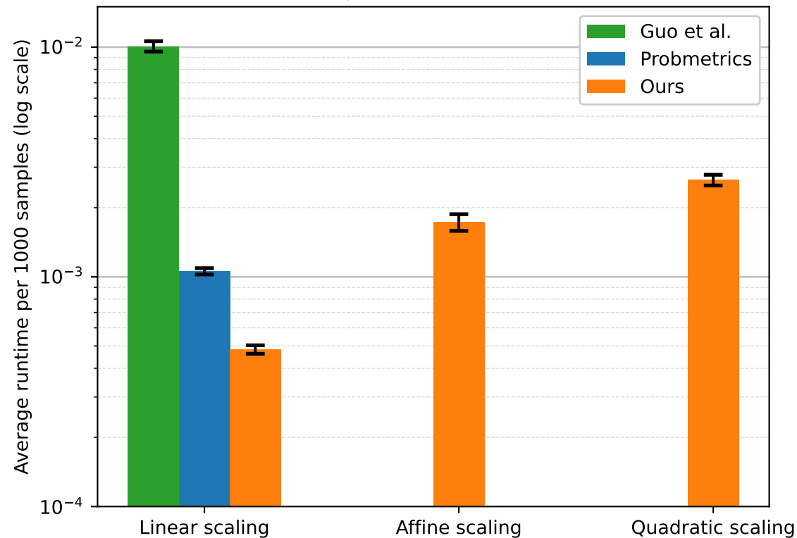
Speed benchmark
