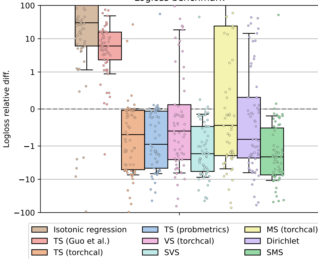
Logloss benchmark
