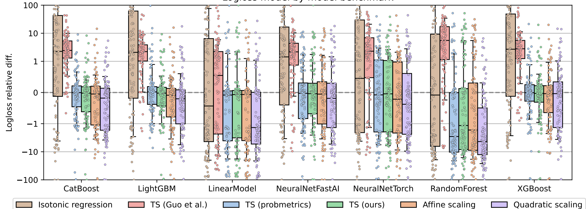
Logloss model by model benchmark
