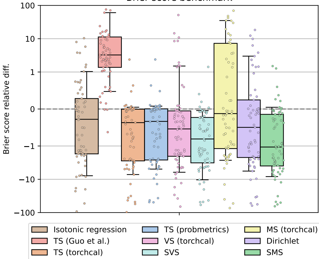
Brier score benchmark
