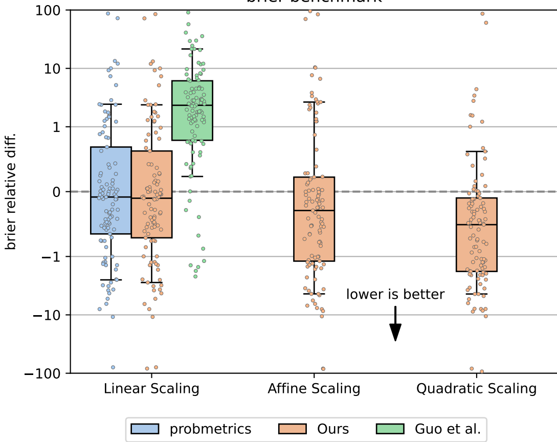
brier benchmark
