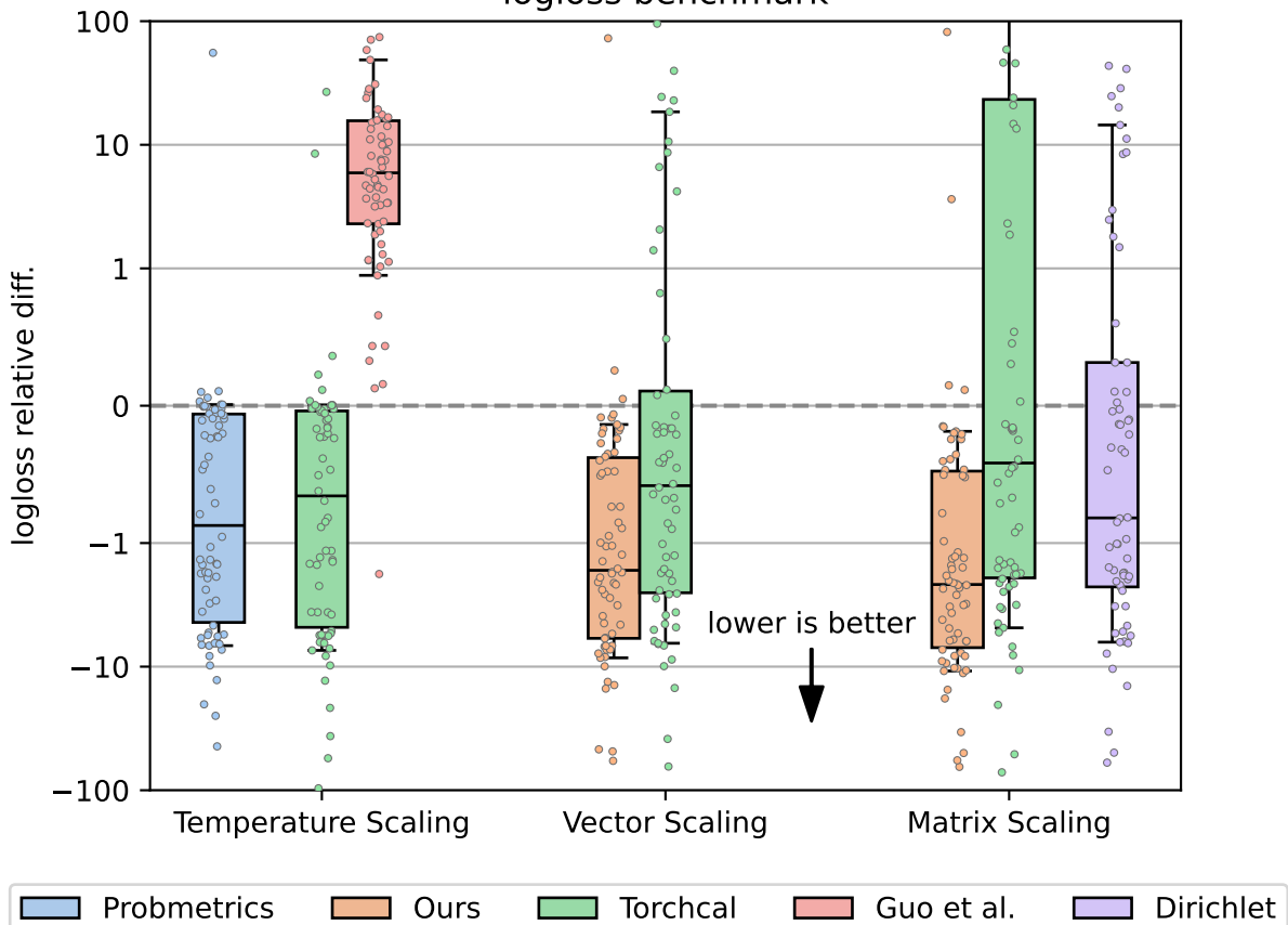
logloss benchmark
