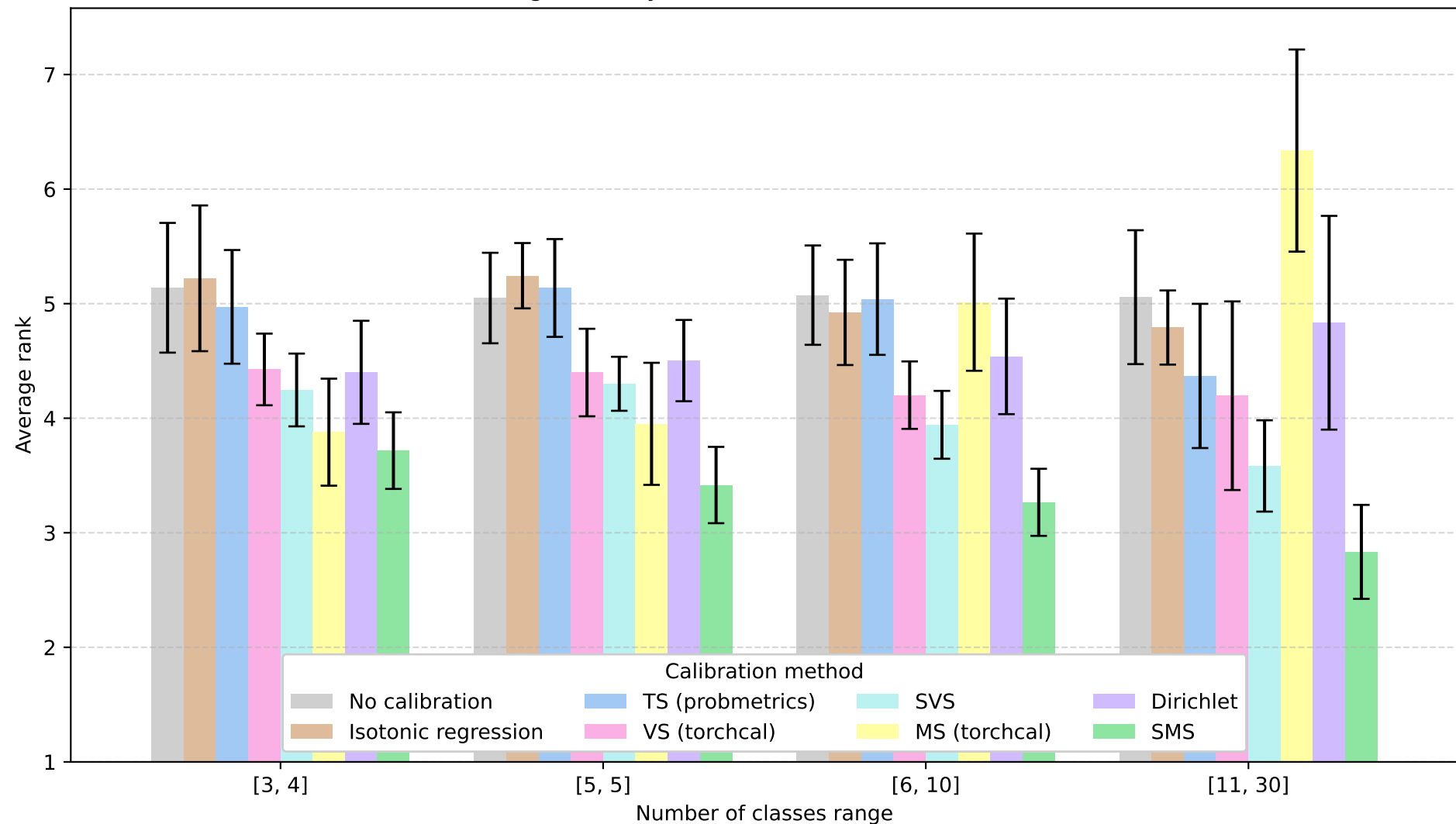
Average rank by number of classes (with 95% CI)
