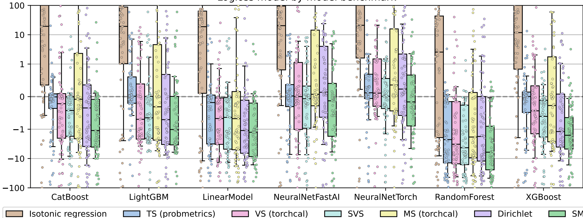
Logloss model by model benchmark
