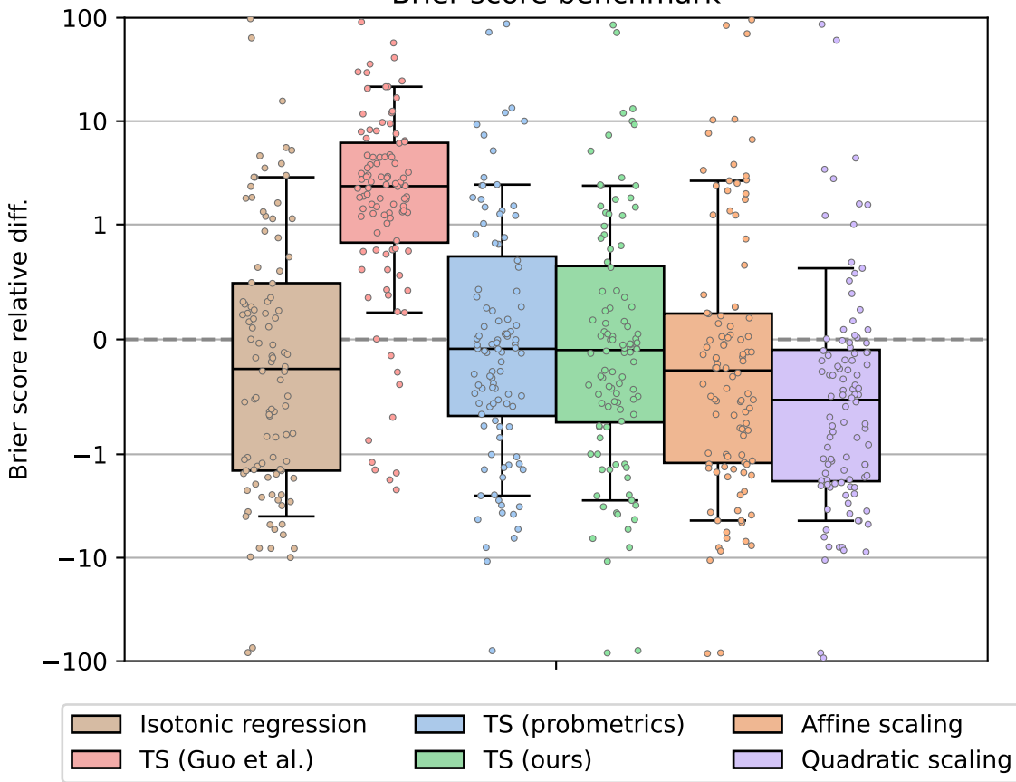
Brier score benchmark
