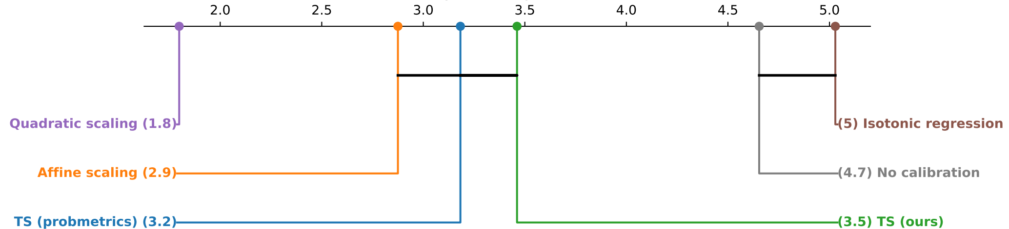
Critical difference diagram of logloss after calibration ranks
