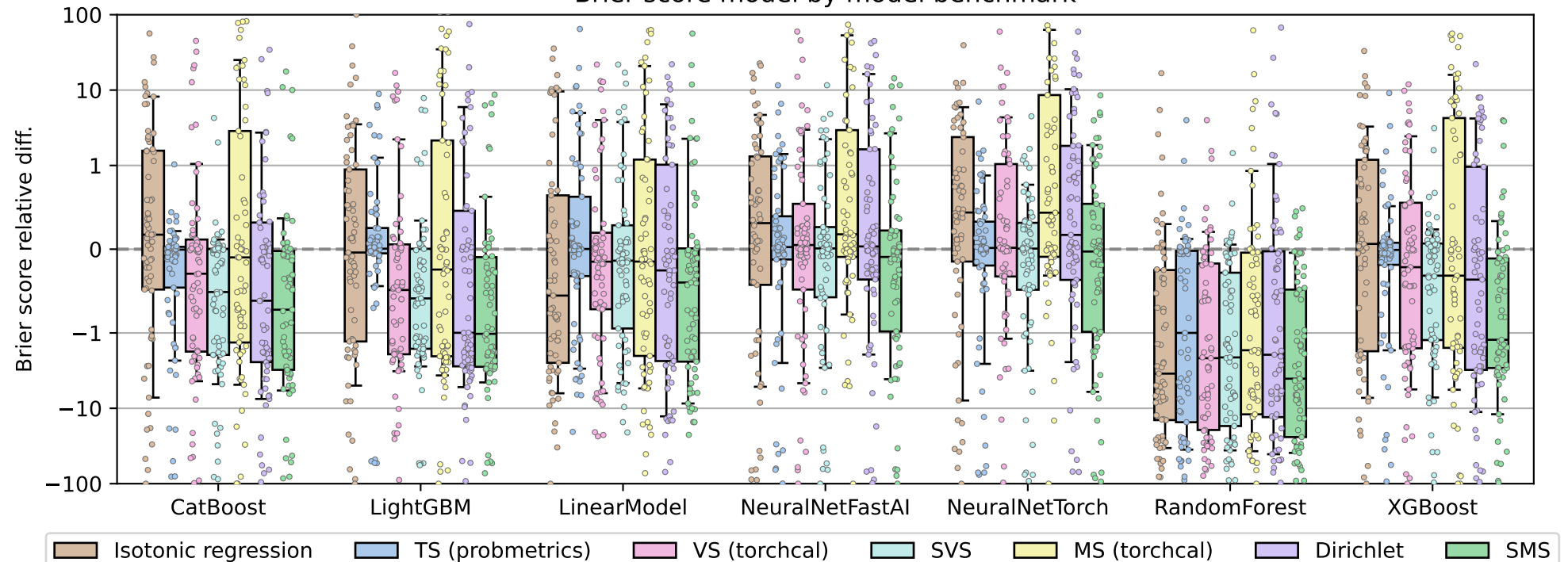
Brier score model by model benchmark
