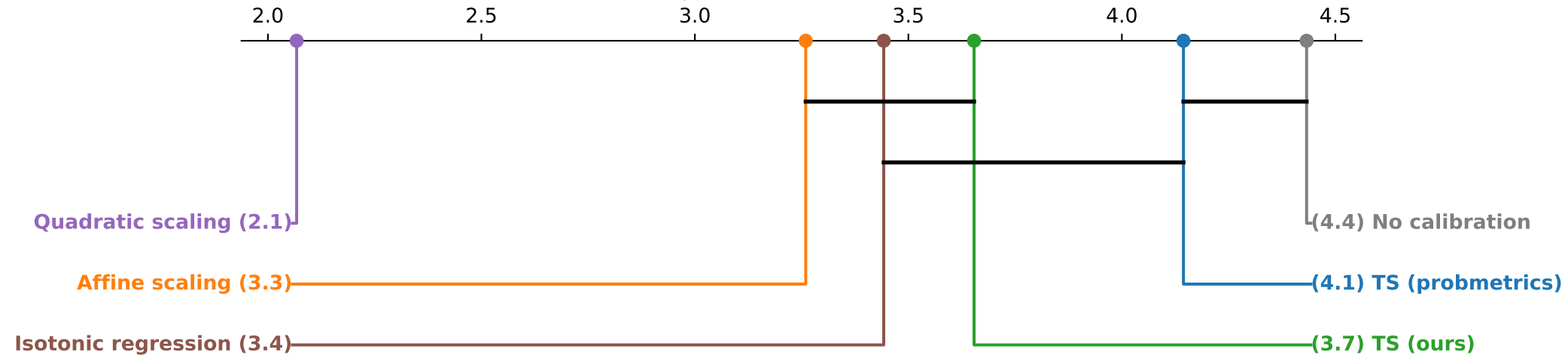
Critical difference diagram of Brier score after calibration ranks
