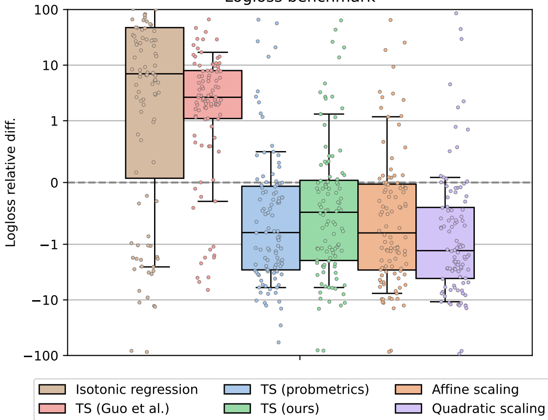
Logloss benchmark
