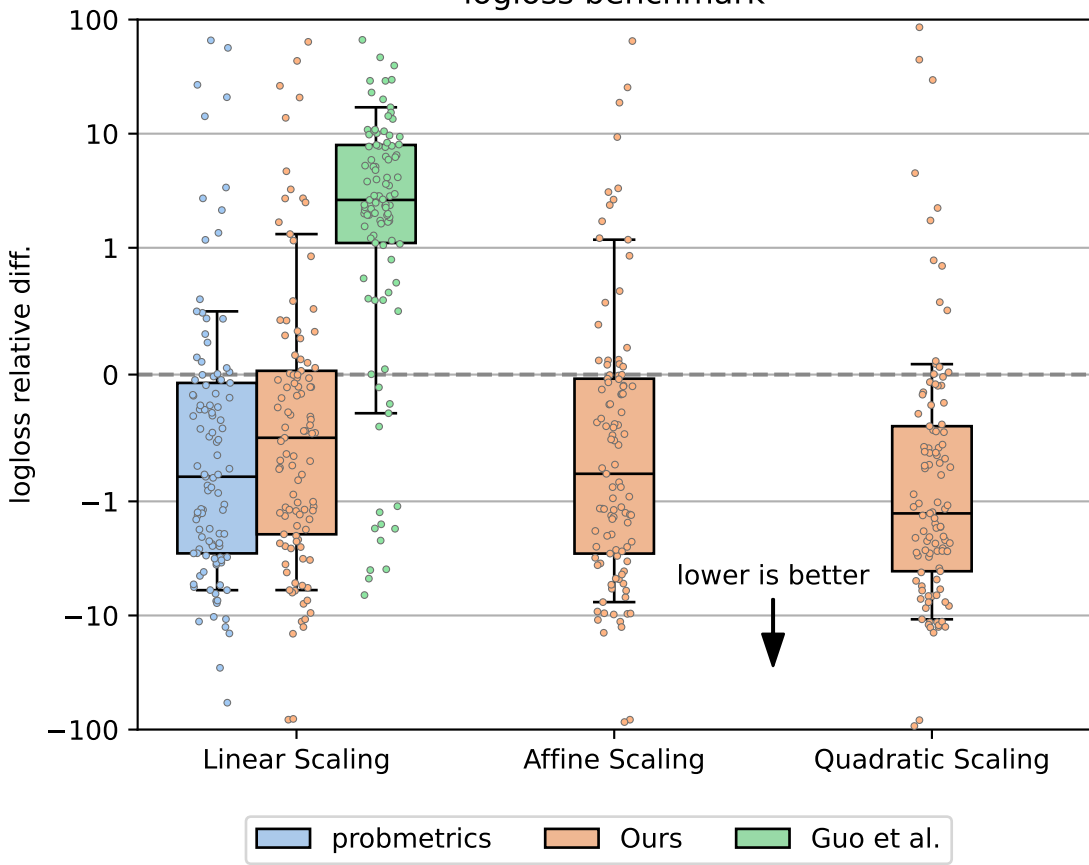
logloss benchmark
