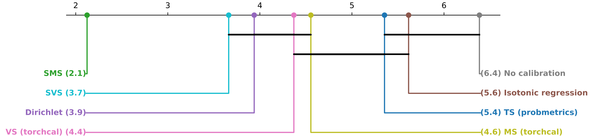
Critical difference diagram of Brier score after calibration ranks
