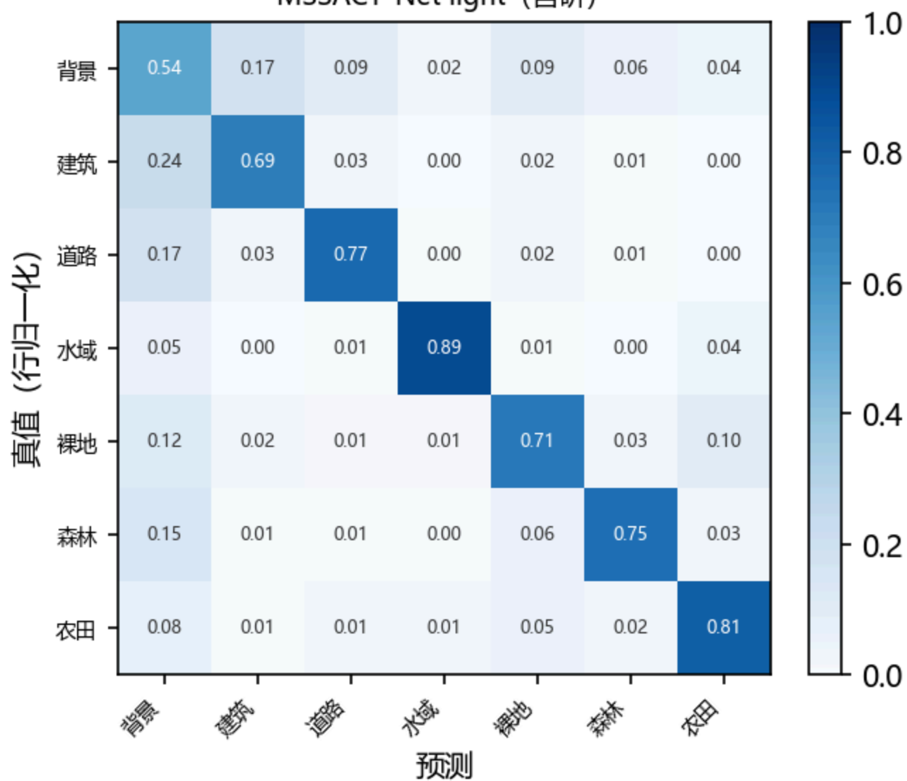
MSSACT-Net light (自研)
