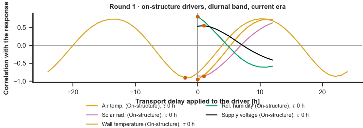
Figure 2: Round 1. Correlation against lag for each on-structure driver, diurnal band, current era. The marked point on each curve is the optimum the scan selected. The supply voltage is drawn with the rest: it is the negative control, and its curve is the floor the others are read against.
