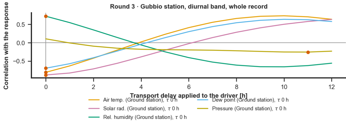
Figure 4: Round 3. Correlation against lag for the Gubbio station channels, diurnal band, whole record.
