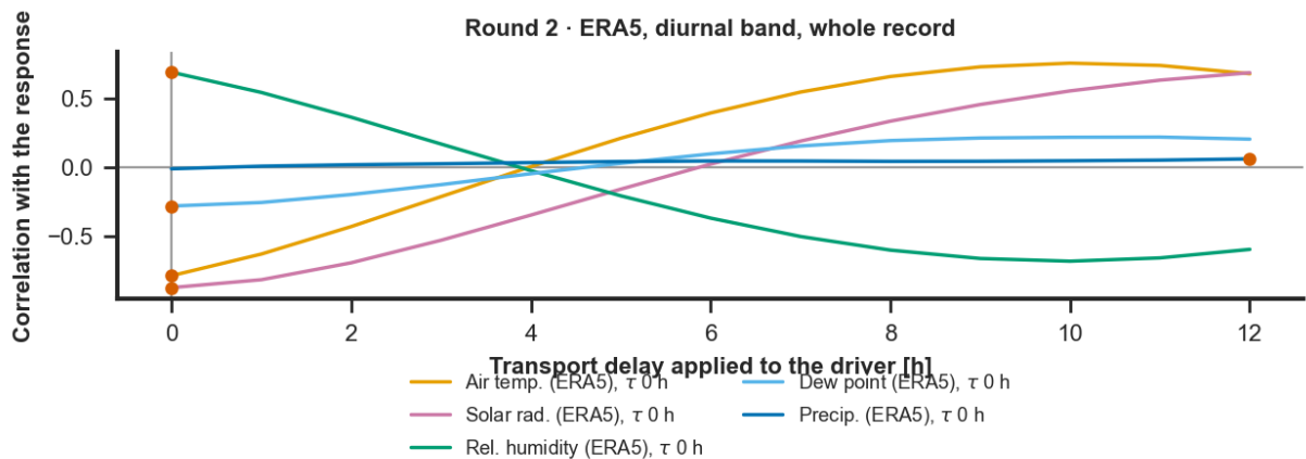
Figure 3: Round 2. Correlation against lag for the ERA5 channels, diurnal band, whole record.
