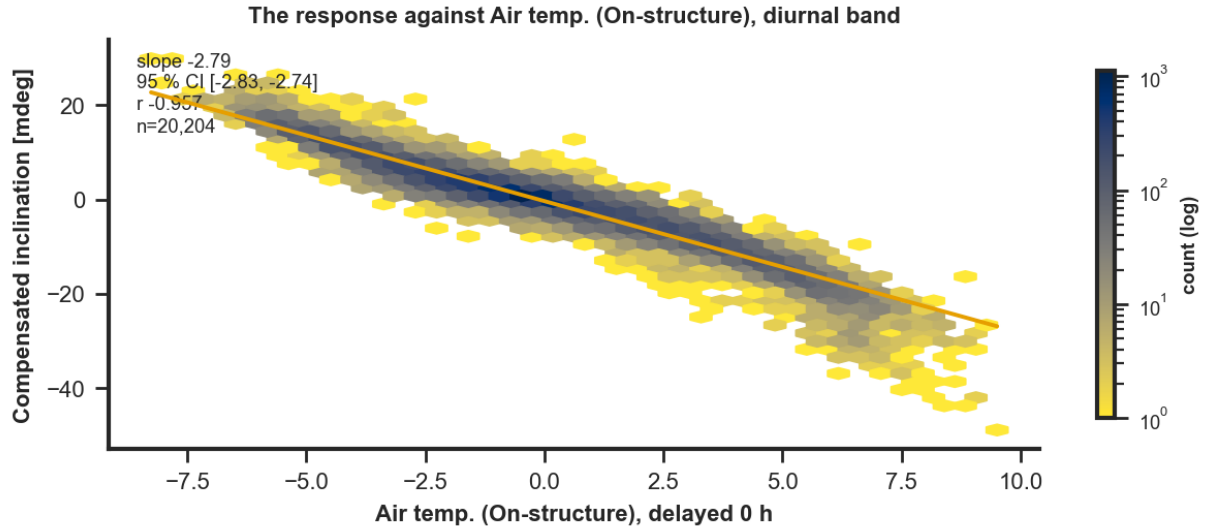
Figure 8: The response against the strongest surviving driver at the lag the scan selected, diurnal band, with the fitted gain and its interval.
