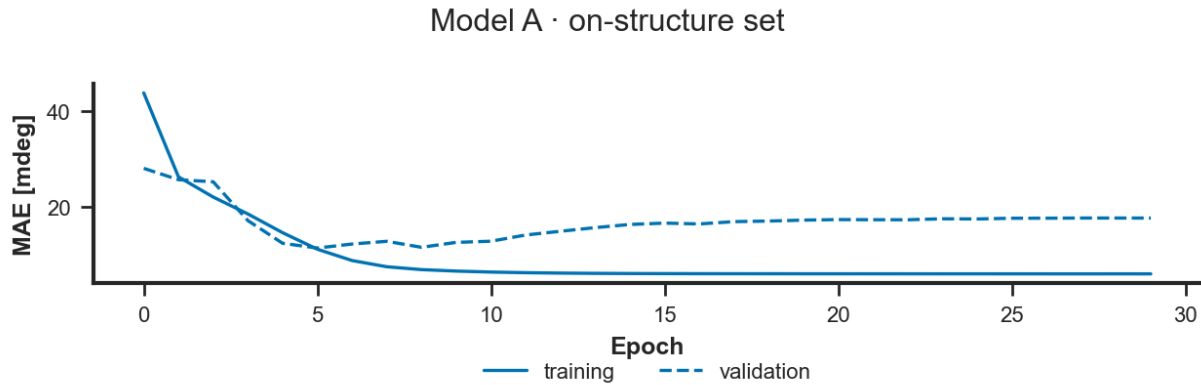
Figure 7: The training curve of the on-structure attribution fit: mean absolute error on the training rows (solid) and on the held-out last fifth (dashed) by epoch, in millidegrees.
