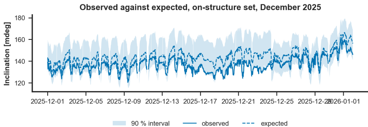
Figure 8: Observed inclination against the rolling expectation with its 90 % conformal interval, on-structure set, December 2025, on the twenty-minute grid.
