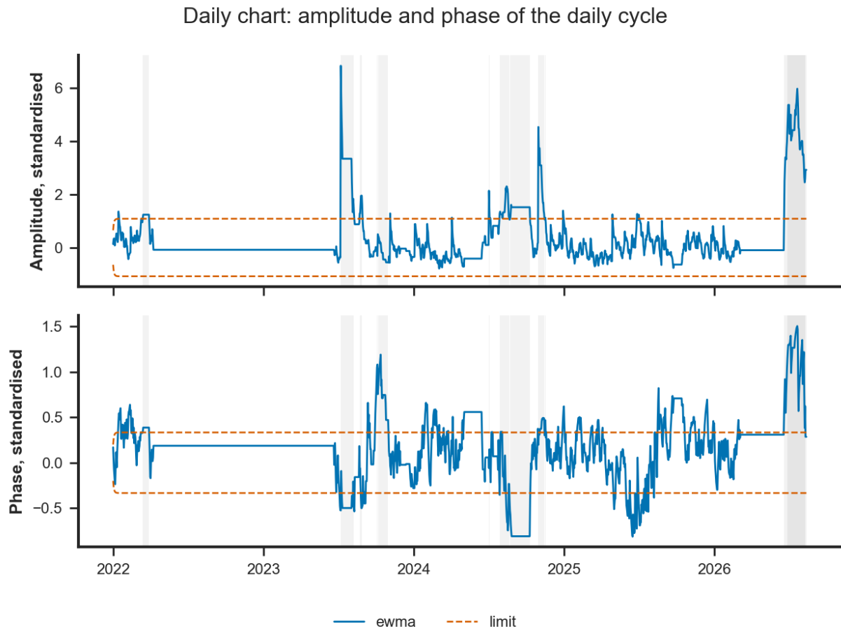
Figure 12: The daily chart: the amplitude (top) and phase (bottom) of the 24-hour harmonic fitted to each day’s residual, standardised on the reference window, with their tuned limits and their episodes shaded.
