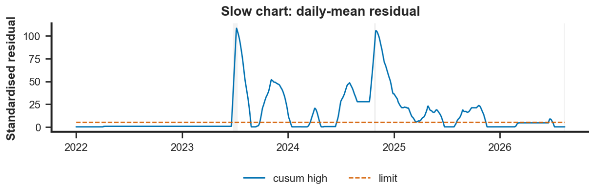
Figure 13: The slow chart: the upper CUSUM of the daily mean residual against its decision interval, episodes shaded.
