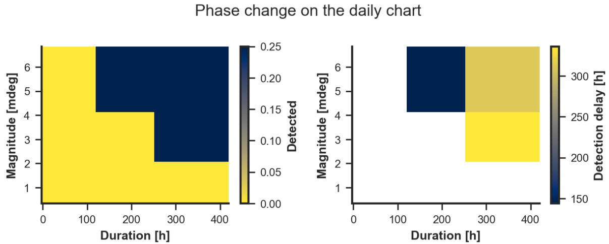
Figure 15: Phase change on the daily-phase chart, the timing shift expressed as the residual amplitude the wall's fitted daily response gives it.
