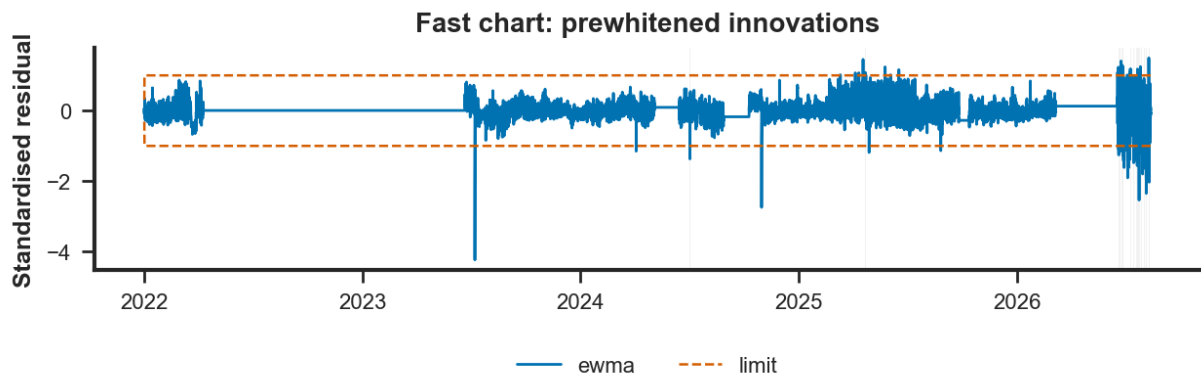
Figure 11: The fast chart over the monitored record: the exponentially weighted moving average of the prewhitened innovations, standardised on the reference window, with the tuned limit; alarming episodes shaded. The average keeps its last value where the residual is missing, so the line runs flat across a gap and an alarm raised before a gap persists through it.
