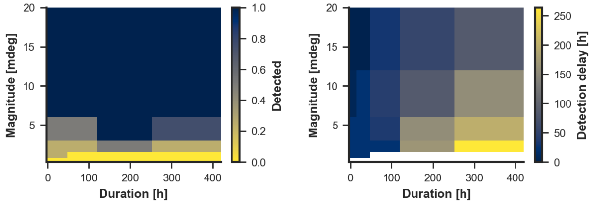
Figure 14: Amplitude growth on the daily-amplitude chart: the fraction of injection dates detected (left) and the mean detection delay (right) by magnitude and duration.
