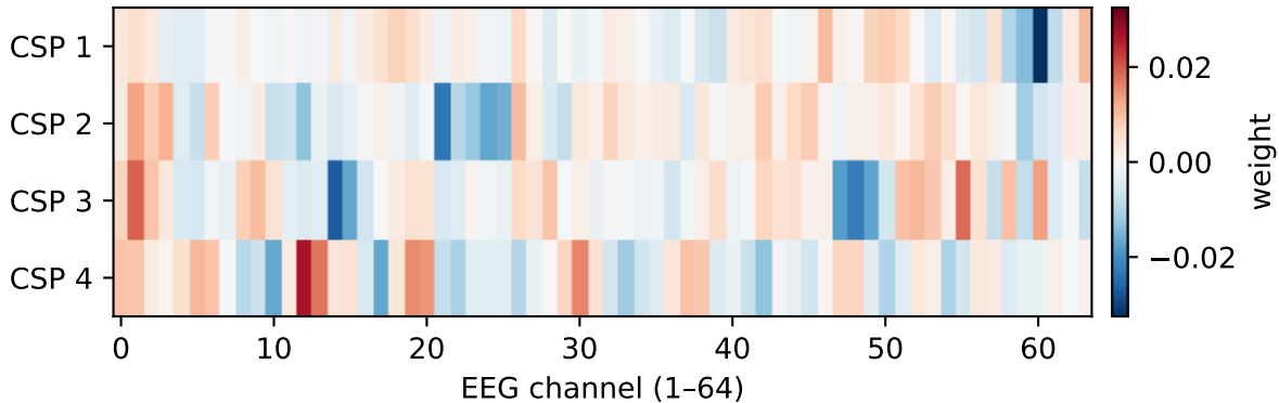
S001 CSP spatial filters (4 components \times 64 channels)
