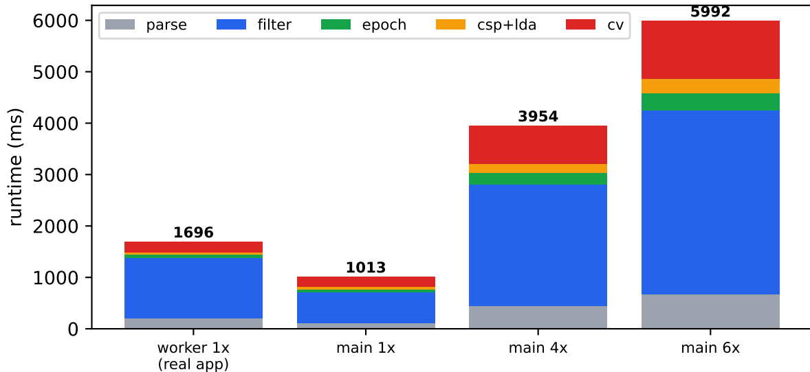
Pipeline runtime (Apple M4, Chromium 148.0.7778.96, n=12) main 4x/6x = CPU-throttled PROXY, not a physical device
