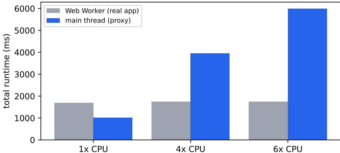
CDP CPU throttling reaches the main thread but NOT Web Workers (worker ~flat; main-thread proxy scales ~1/4/6x)
