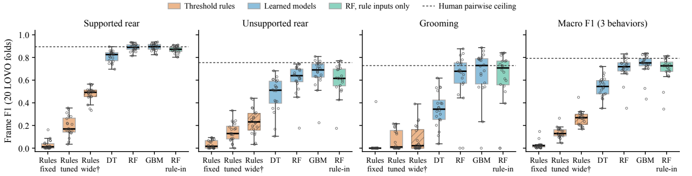
Fig. 2. Per-behavior frame F1 over the 20 LOVO folds. Each open circle is one held-out video; boxes give the median and quartiles and whiskers reach the furthest video within 1.5 IQR. Color marks the method family (legend); the hatched box is the post-hoc wide grid. Dashed line: mean pairwise F1 between the three human raters.
