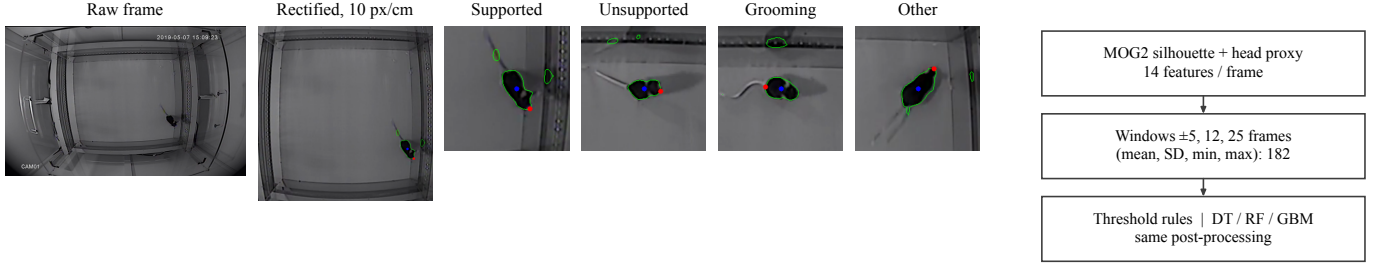
Fig. 1. Pipeline. Frames are rectified to a metric top-down canvas; MOG2 gives a silhouette (green contour, blue centroid), from which 14 features, including a contour head proxy (red), are computed; window statistics feed either threshold rules or a learned classifier, with identical post-processing. Crops show consensus examples from one video.
