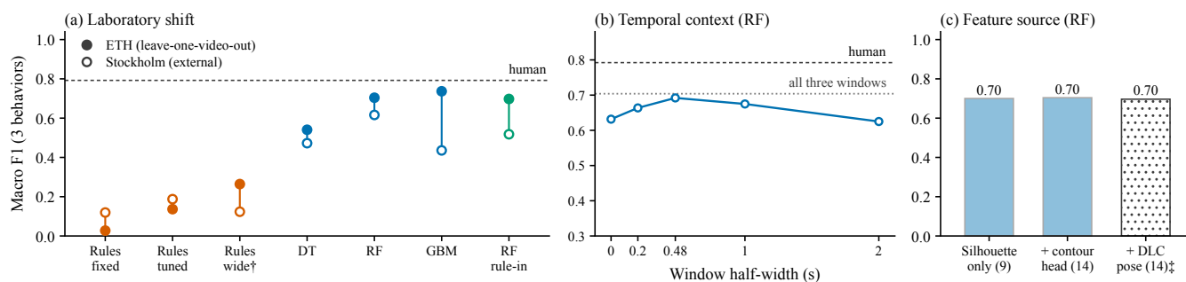
Fig. 3. (a) Macro F1 on ETH (filled markers, mean over the 20 folds) and on the external Stockholm set (open markers), joined per method. (b) RF on the raw features plus a single window of the given half-width; the dotted line is the pre-registered three-window model. Note the zoomed vertical axis in (b); (a) and (c) span the full range. (c) RF by feature source; †DeepLabCut features come from the original study (GPU-trained), shown as a reference rather than as a competing system. Dashed line: mean pairwise F1 between the three human raters.
