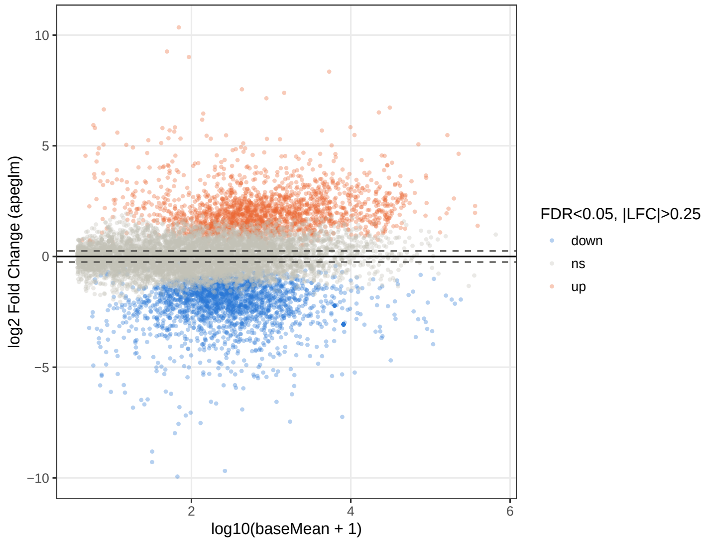
MA plot – SKTI vs_Control
