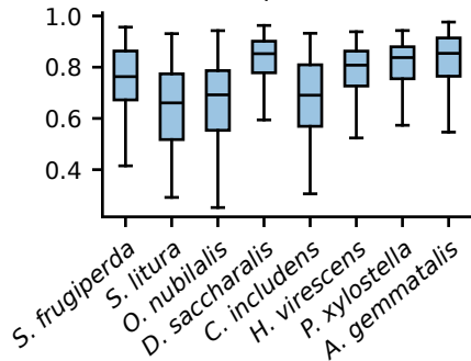
ipTM
