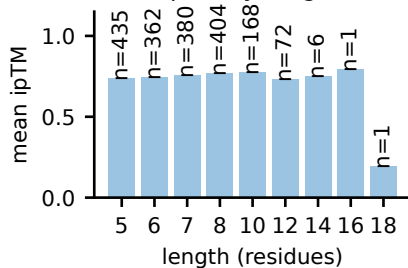
ipTM by length
