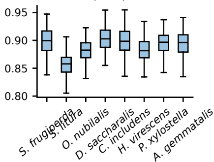
complex pLDDT
