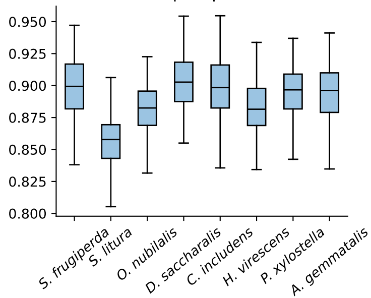
complex pLDDT
