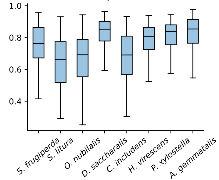
ipTM
