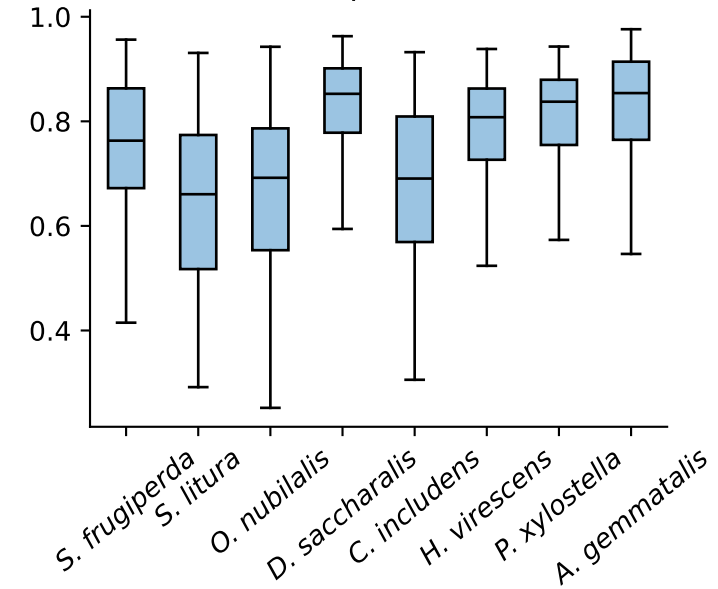
ipTM
