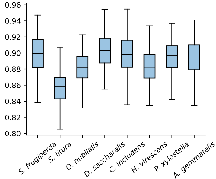
complex pLDDT
