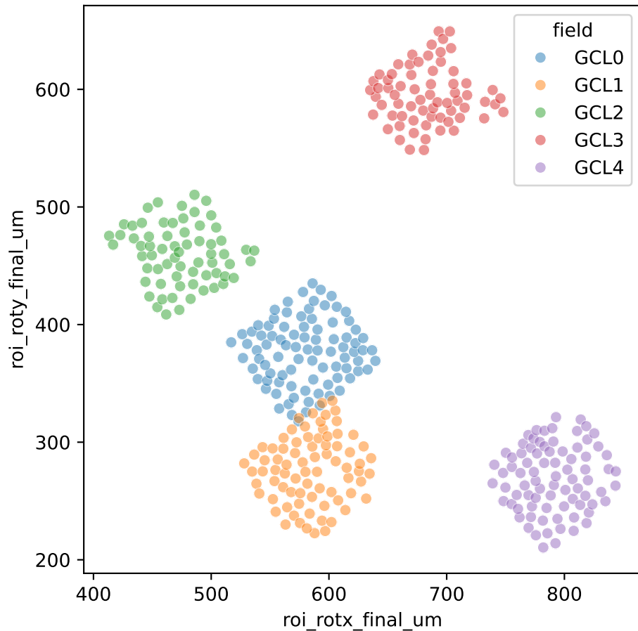
2p coordinates, global + per-field alignment
