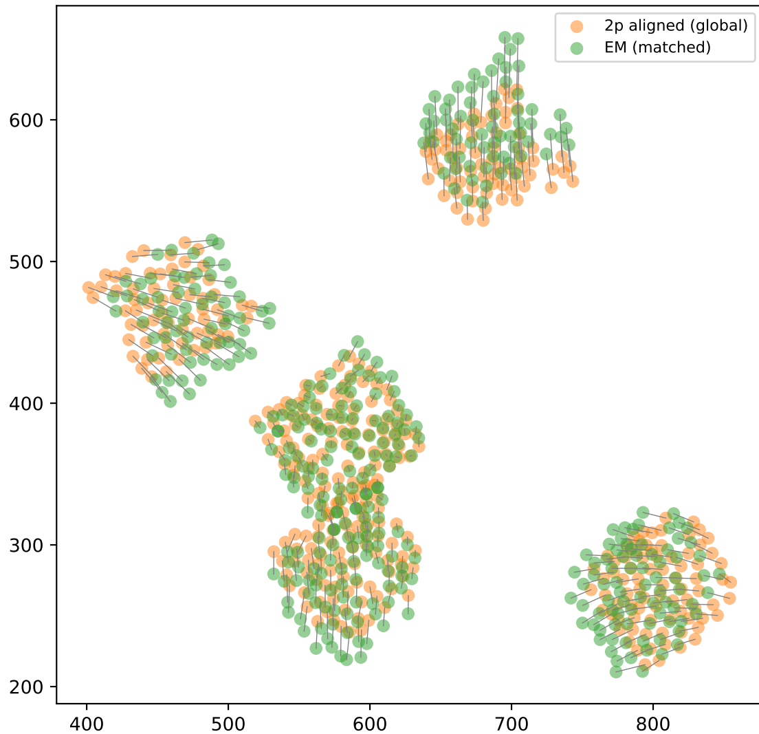
Global alignment RMSE=15.6 \mu\text{m}
