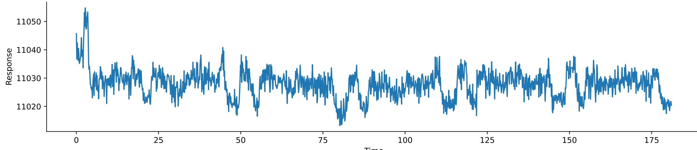
Raw chirp response
