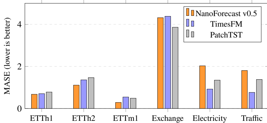
Figure 2: MASE by dataset (lower is better). v0.5 (orange) leads on the three ETT sets and stays close on exchange rate; TimesFM leads the two high-cardinality sets.
