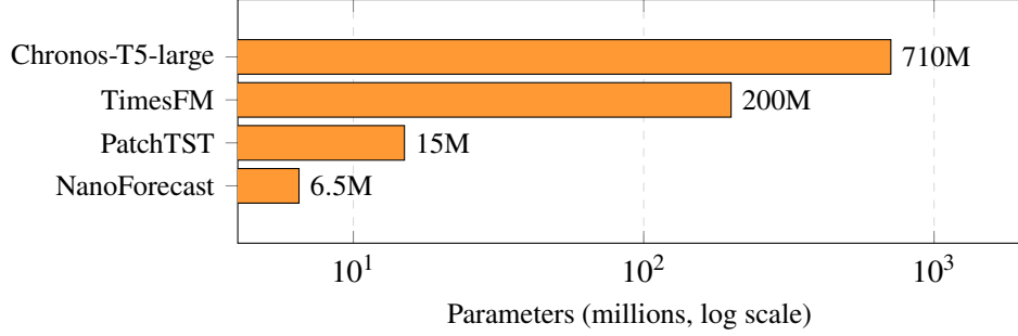
Figure 3: Parameter counts (log scale). NanoForecast v0.5 uses 31× fewer parameters than TimesFM and 109× fewer than Chronos-T5-large.
