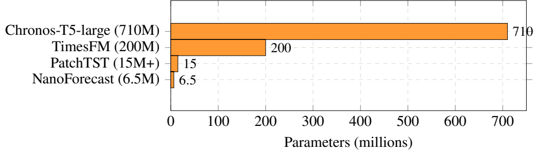
Figure 3: Parameter count comparison. NanoForecast v0.5 (6.5M) is 31\times smaller than TimesFM (200M) and 109\times smaller than Chronos-T5-large (710M).
