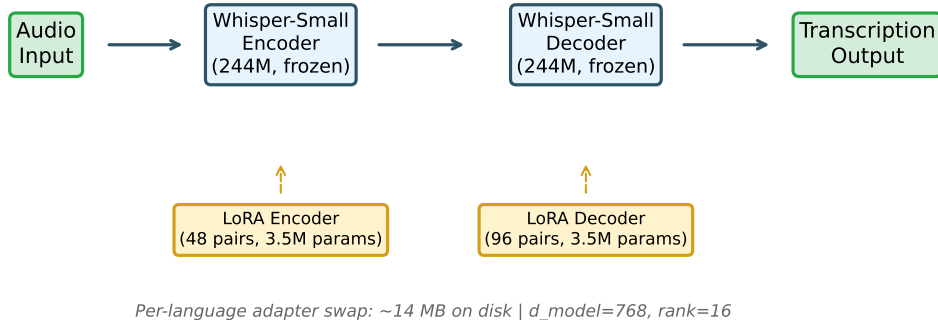
Figure 1: Architecture. A single frozen Whisper-Small backbone serves all five languages. Per-language LoRA adapters (rank 16, ~14 MB each) are injected via forward hooks on every attention projection. Switching languages swaps hooks with no weight reloading. ONNX exports fuse the chosen adapter into the graph for CPU inference.
