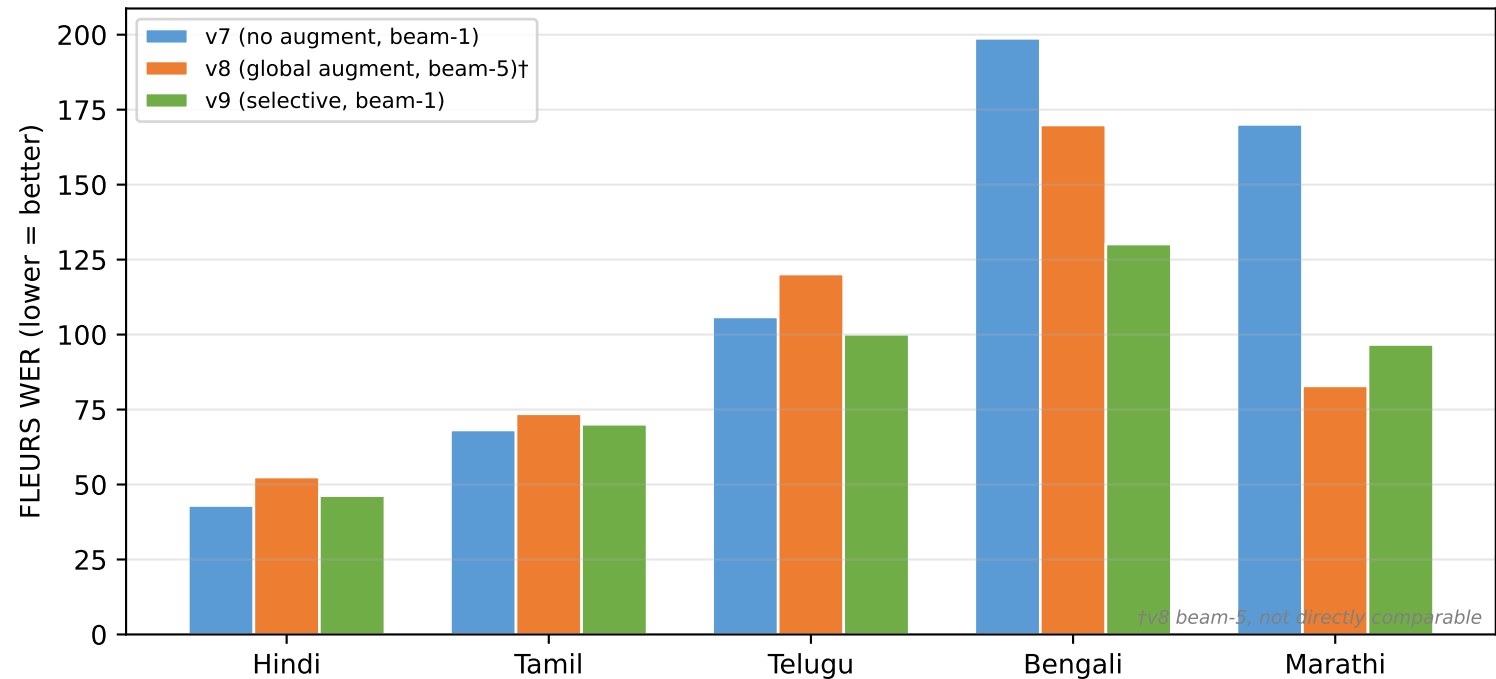
PolyWhisper: v7 vs v8 vs v9
