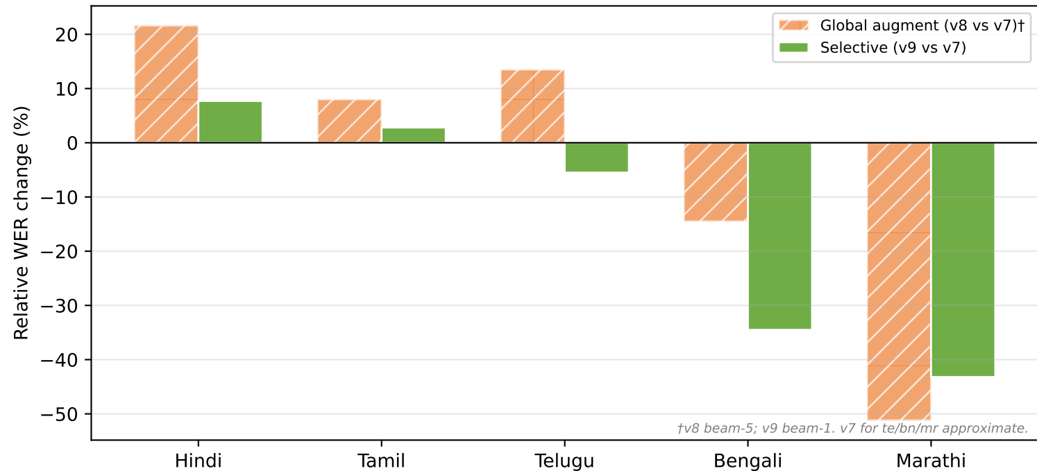
Augmentation Asymmetry: v7→v8 (global) vs v7→v9 (selective)
