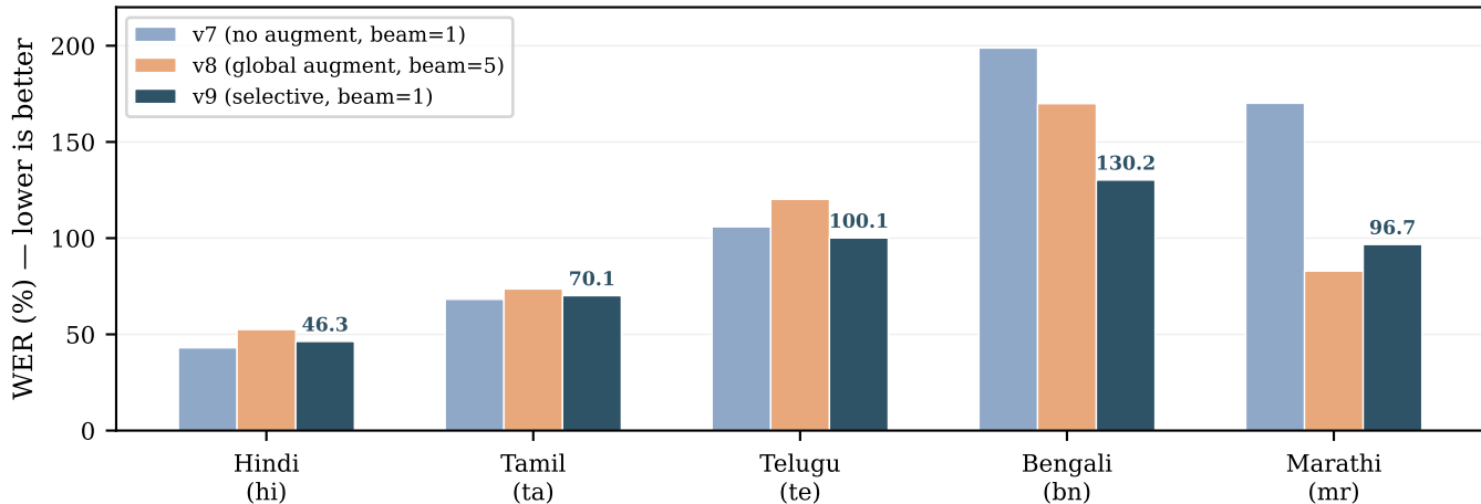
PolyWhisper WER across training variants (FLEURS test, normalized scoring)
