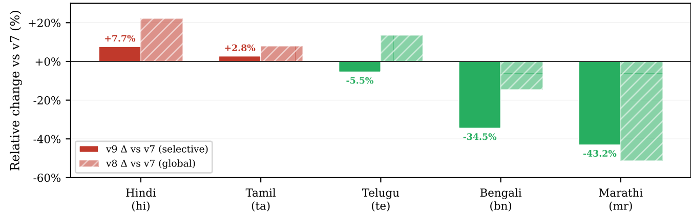
Per-language augmentation asymmetry: selective vs global (negative = improvement)
