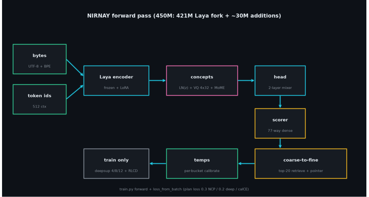
Figure 5: Forward pass: byte path, frozen encoder plus LoRA, concept bottleneck, dense scorer, coarse-to-fine pointer, per-bucket temperatures. Deep supervision and RLCD exist only in training.
