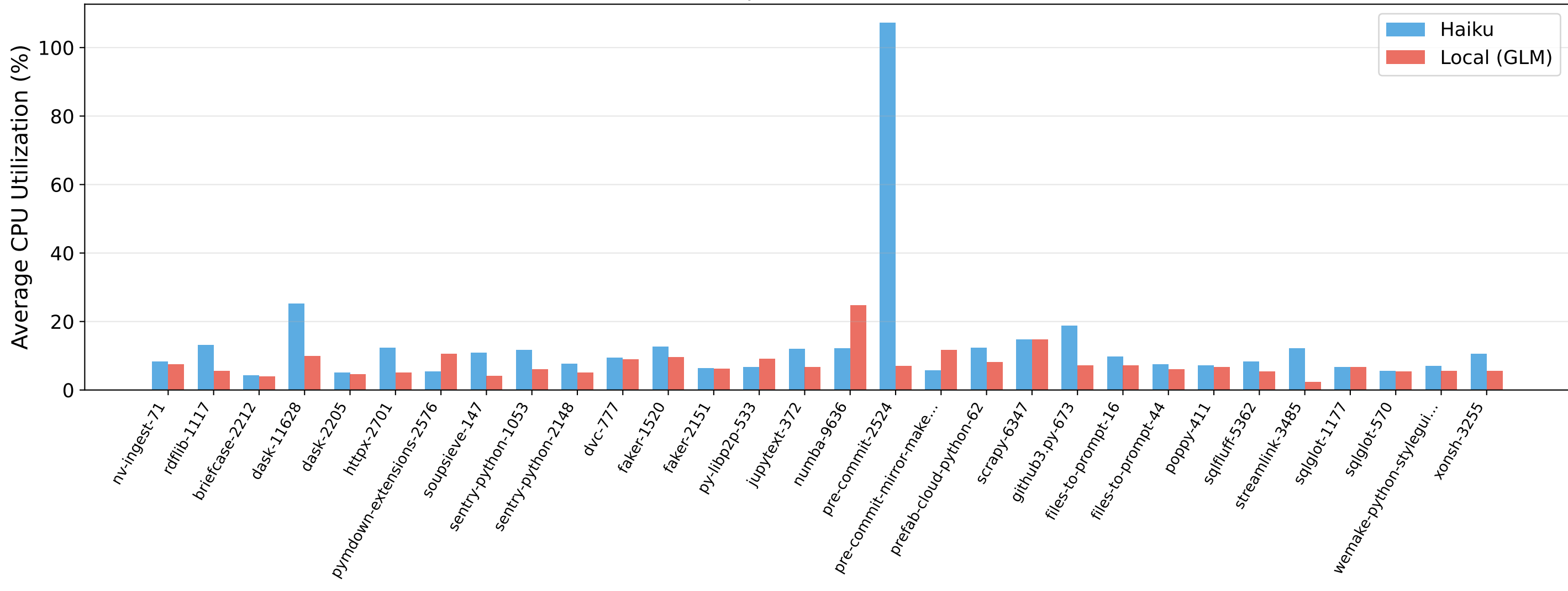
CPU Utilization Comparison: Haiku vs Local (30 tasks)
