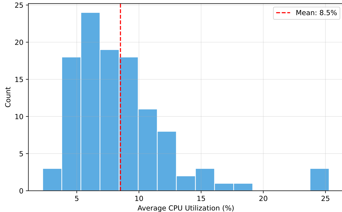
CPU Utilization Distribution
