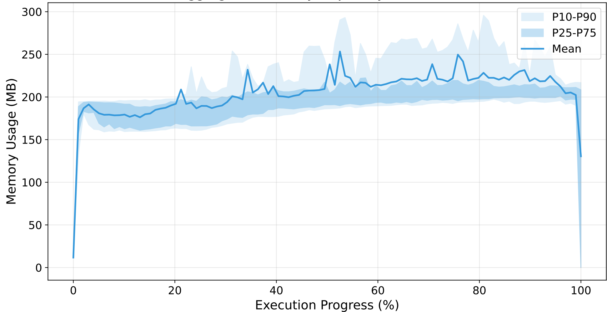
Aggregated Memory Trajectory (n=33 tasks)
