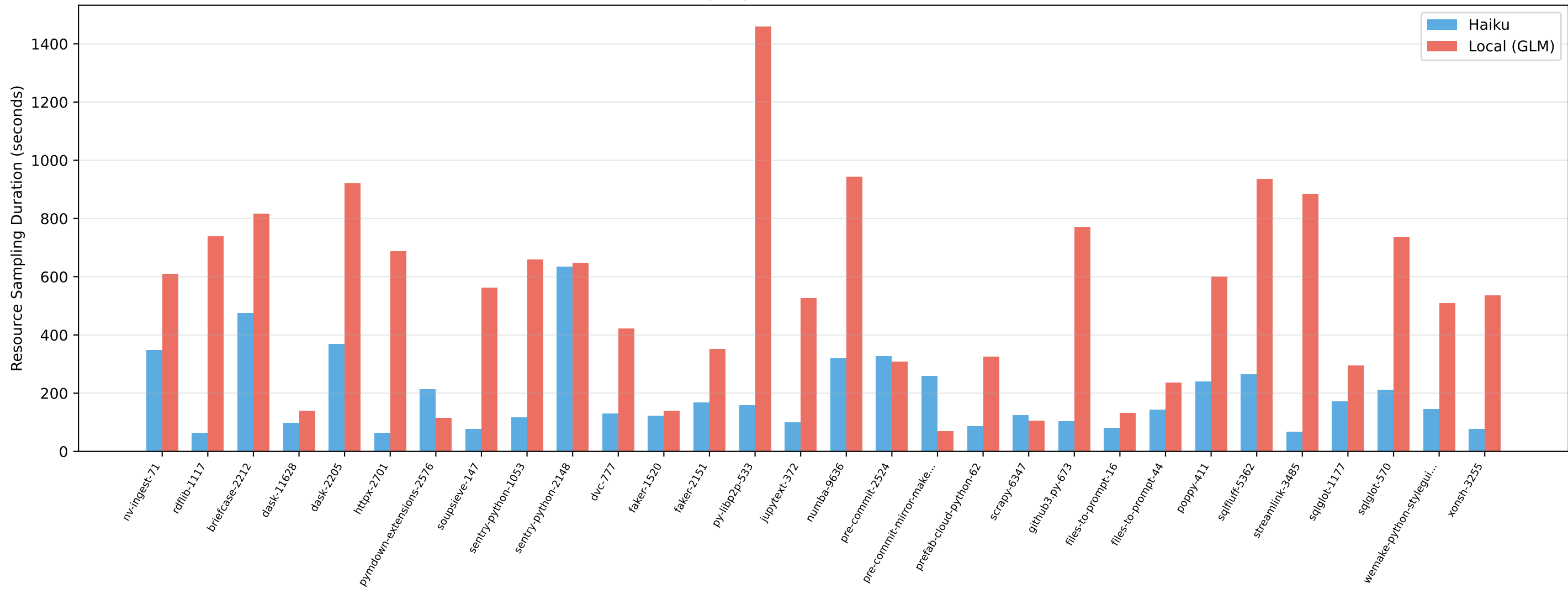
Resource Sampling Duration: Haiku vs Local (30 tasks)
