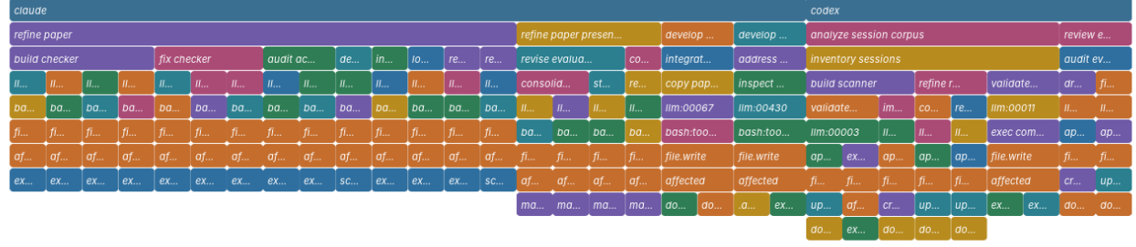
Figure 6: FILE-WRITE view of the same self-profile hierarchy. Width is target-reference count, with each created file preserved along the semantic operation → LLM → tool → exact write-target path.
