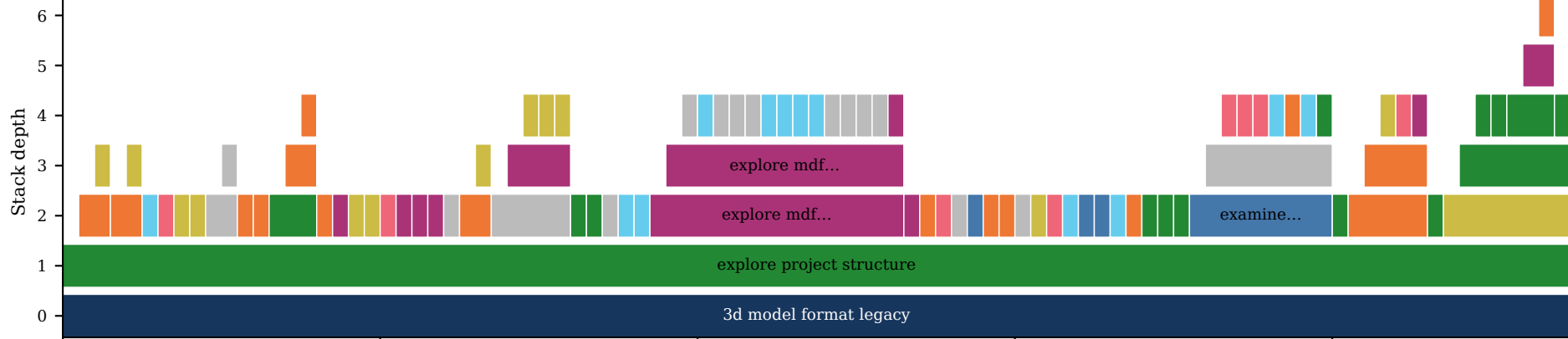
(b) After support-at-least-two contraction
