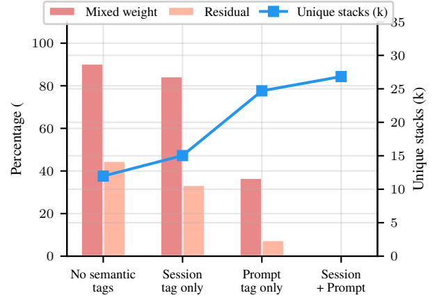
Figure 3: RQ1 semantic-axis ablation on 183,714 system observations from 325 real trajectories. Bars show mixed weight and residual percentages on the left axis, and the line shows unique stacks on the right axis. Adding prompt tags reduces mixed weight from 90.4% to 36.7% while increasing unique stacks from 12k to 25k. Session tags alone barely help (84.4%).
