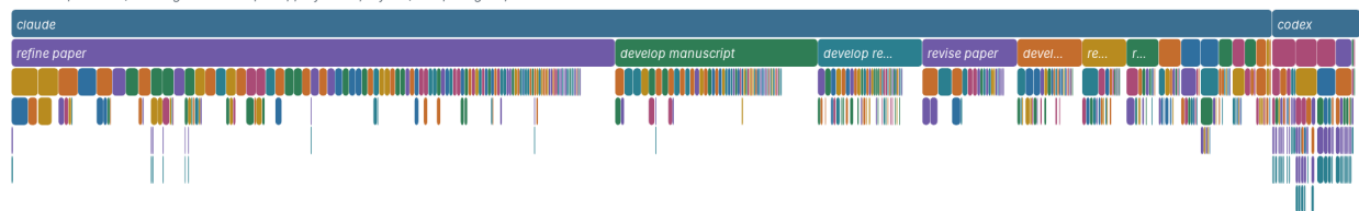
Figure 4: The complete 42-session development population under one fixed semantic hierarchy. Width is provider-reported tokens (top) or operation count (bottom); second-level frames are the annotated responsibilities ( refine paper , develop manuscript , develop research , ...), with deeper refinements and source labels available for drilldown in stock pprof.
