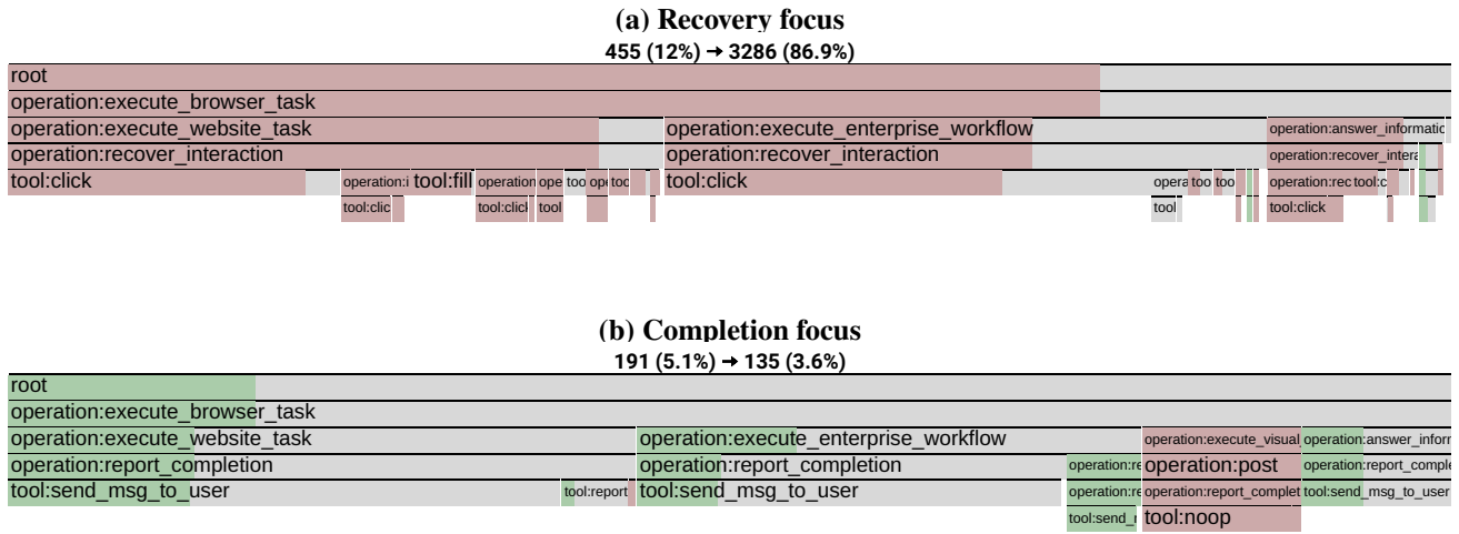
Figure 4: Stock-pprof differential flamegraphs over all 338 bad–good pairs. Each box width is the sum of the good/base and bad/candidate contributions; the inset is their net bad-minus-good difference (rose: more in bad; green: more in good; gray: overlapping remainder). The arrow reports good → bad, with percentages relative to the 3,780-operation good diff base. Recovery grows from 455 to 3,286 occurrences (net +2,831); completion falls from 191 to 135 (net −56). Agent and source-call frames are hidden only in this display; the signed pprof retains them and their evidence labels. These are aggregate diagnostic differences, not causal effects.
