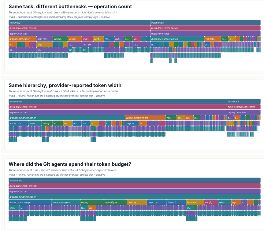
Figure 2: All three real git-multibranch executions under one fixed operation hierarchy. Width is operation count (top) or provider-reported tokens (middle); the bottom panel focuses the shared diagnose authentication operation. AgentPProf emits only standard pprof; a paper-only renderer reads the same .pb.gz through go tool pprof without introducing a product frontend.
