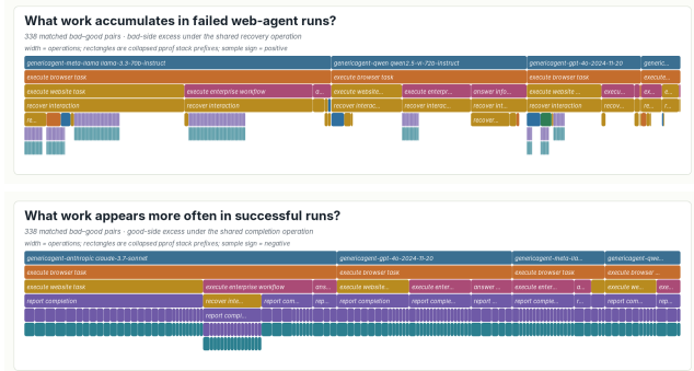
Figure 3: Focused paper renderings of the signed pprof profile over all 338 bad-good pairs. The top panel selects positive samples under recover interaction: 3,286 bad-side versus 455 good-side occurrences. The bottom selects negative samples under report completion : 135 bad-side versus 191 good-side occurrences. These are aggregate diagnostic differences, not causal effects.
