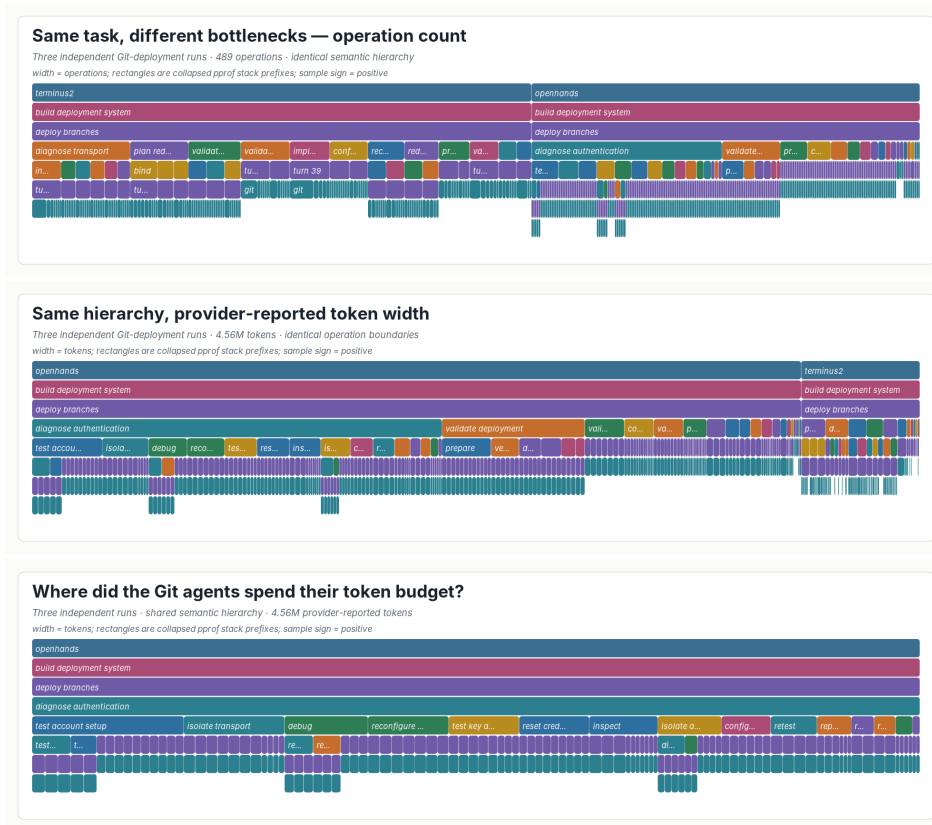
Figure 2: All three real git-multibranch executions under one fixed operation hierarchy. Width is operation count (top) or provider-reported tokens (middle); the bottom panel focuses the shared diagnose authentication operation. AgentPProf emits only standard pprof; a paper-only renderer reads the same .pb.gz through go tool pprof without introducing a product frontend.
