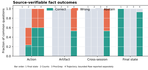
Figure 2: Correct, wrong, and abstaining outcomes on the corrected 120-question oracle for the deterministic conditions. Bounded Raw is evaluated separately under the registered fixed-reader protocol.
