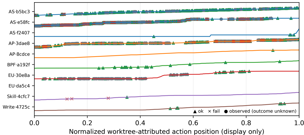
A. Worktree action trajectories
