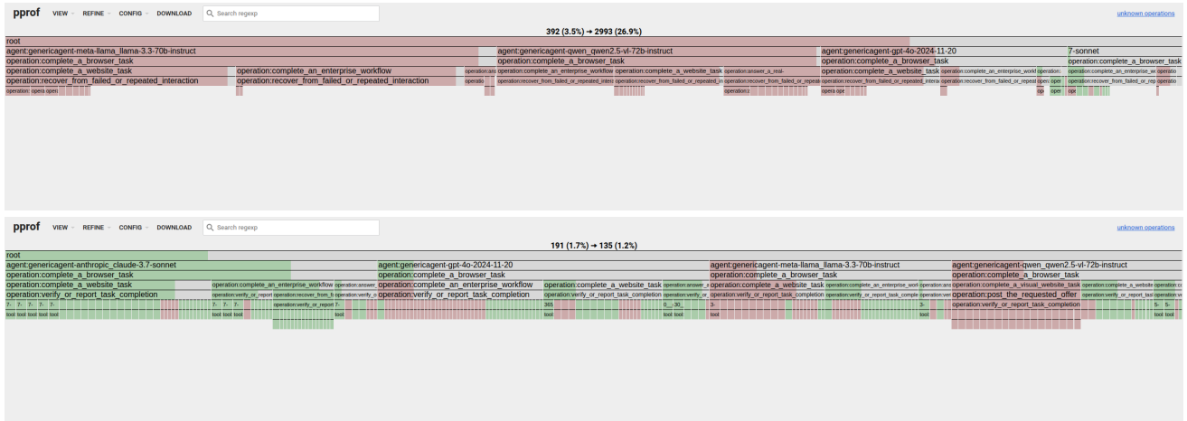
Figure 3: Focused stock-pprof views of the signed differential profile over all 338 bad–good pairs. Red is bad-side excess and green is good-side excess. The recursive recovery subtree contains 2,993 bad-side versus 392 good-side occurrences (top); the completion subtree contains 135 bad-side versus 191 good-side occurrences (bottom). Each path descends from shared responsibilities to the contributing LLM and tool calls. These are aggregate diagnostic differences, not causal effects.
