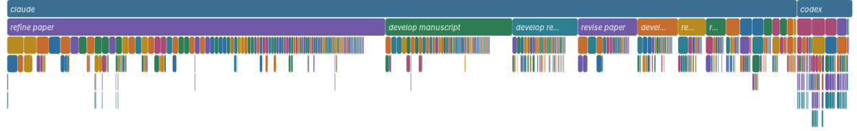
Figure 5: The complete 42-session population under one fixed semantic hierarchy. Width is provider-reported tokens (top) or operation count (bottom); second-level frames are the annotated responsibilities (refine paper, develop manuscript, develop research, ...), with deeper refinements and source labels available for drilldown in stock pprof.
