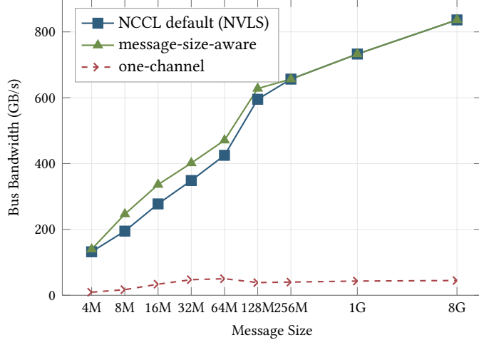
Figure 2. 8-GPU AllReduce on NVLink. The message-size-aware policy selects Ring/LL128 for 4–32 MiB and Ring/Simple for 64–192 MiB, improving throughput by up to 27% over NCCL’s default NVLS algorithm. A one-channel policy shows that a verified program can still degrade throughput.
