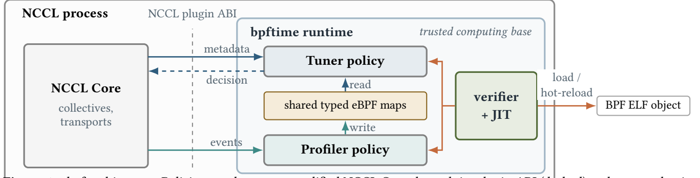
Figure 1. nbpf architecture. Policies attach to an unmodified NCCL Core through its plugin ABI (dashed) and enter only via the verifier and JIT, which serve load and hot-reload. The profiler writes latency into shared maps the tuner reads.
