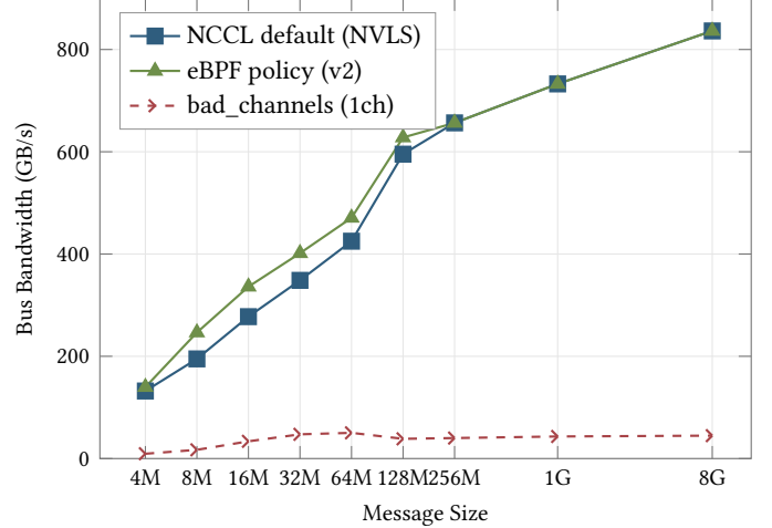
Figure 2. 8-GPU AllReduce on NVLink. The eBPF policy selects Ring/LL128 for 4–32 MiB and Ring/Simple for 64–192 MiB, improving throughput by up to 27% over NCCL’s default NVLS algorithm. A deliberately bad policy (1 channel) shows that policies have real control, including destructive power.
