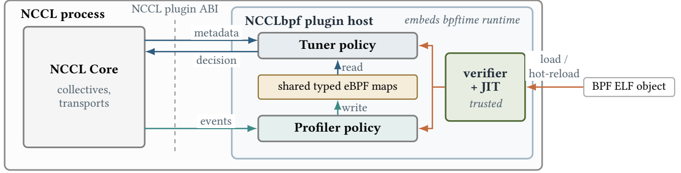
Figure 1. NCCLbpf architecture. The plugin host loads policies in-process, with no external agent: policies attach to an unmodified NCCL Core through its plugin ABI (dashed) and enter only via the verifier and JIT, which serve load and hot-reload. The host, runtime, verifier, and JIT are trusted; the policies are not. The profiler writes latency into shared maps the tuner reads.
