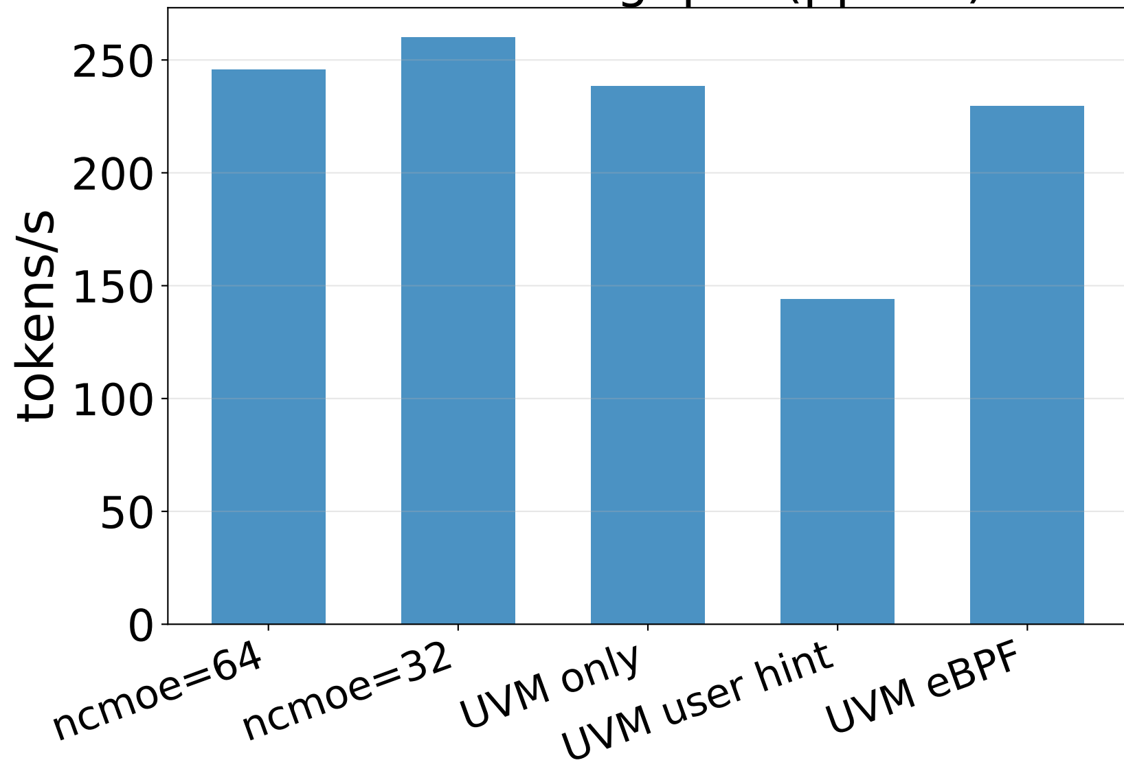
Prefill Throughput (pp512)
