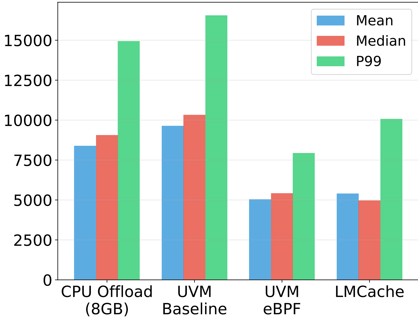
Time to First Token (ms)
