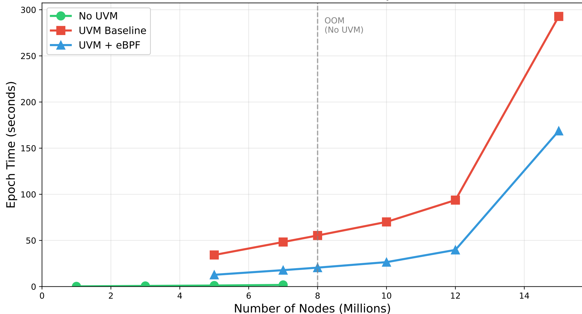
GCN Training: UVM Oversubscription Performance (Without cudaMemPrefetchAsync)
