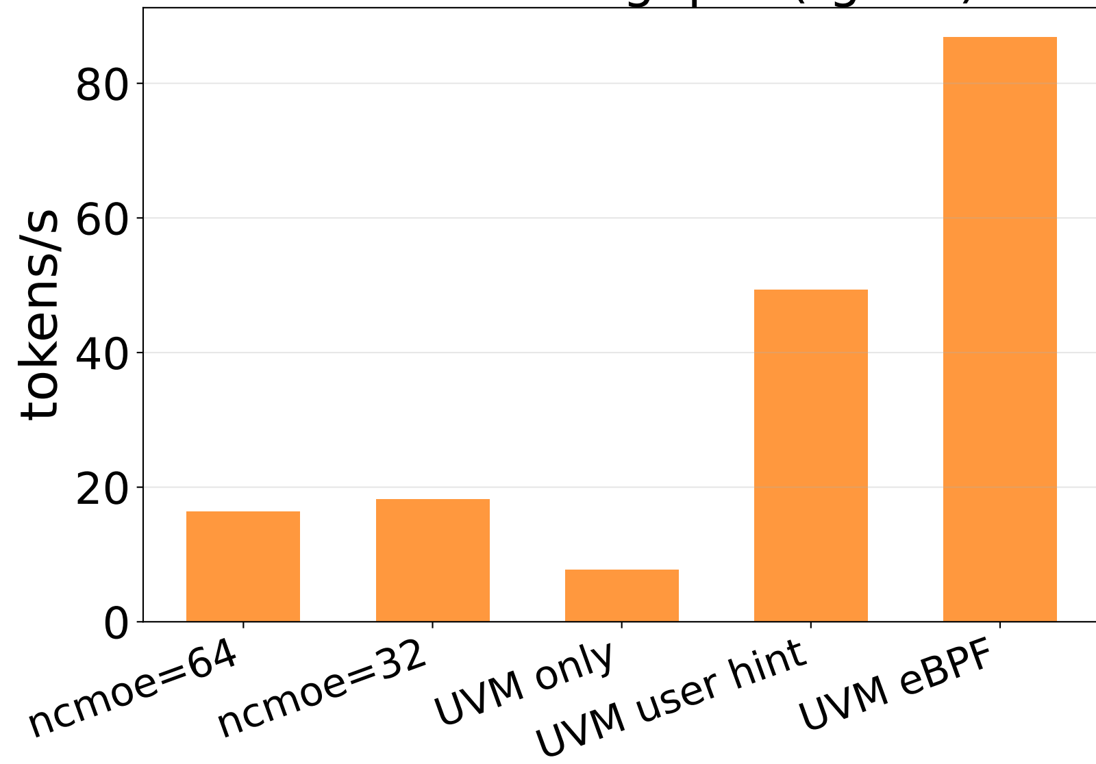
Decode Throughput (tg128)
