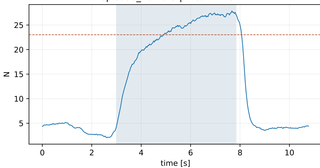
episode_40.hdf5 | mean 22.54 N
