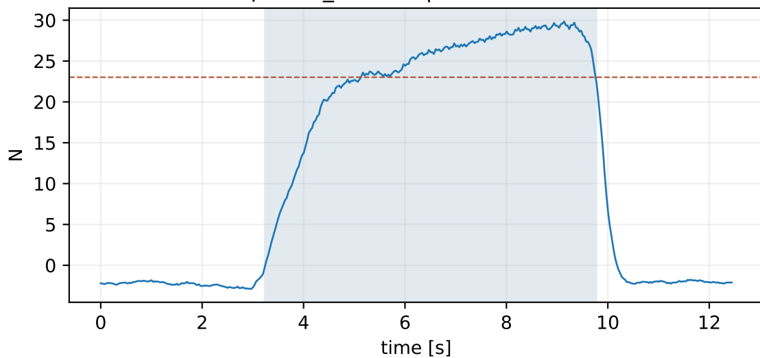
episode_33.hdf5 | mean 23.51 N
