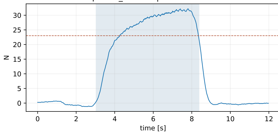
episode_17.hdf5 | mean 25.38 N
