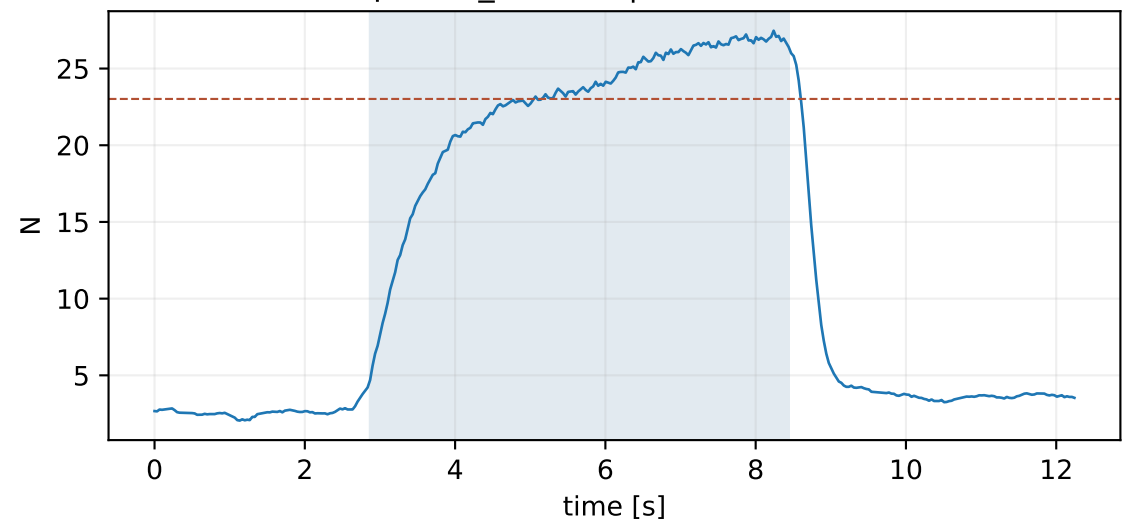
episode_38.hdf5 | mean 22.46 N
