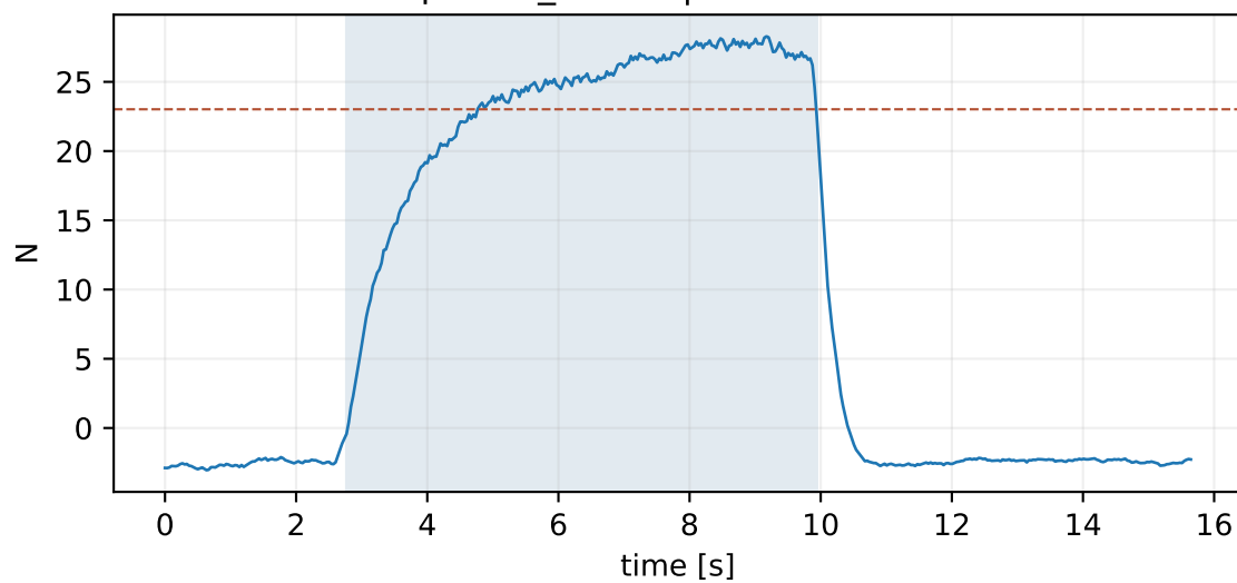
episode_4.hdf5 | mean 23.11 N
