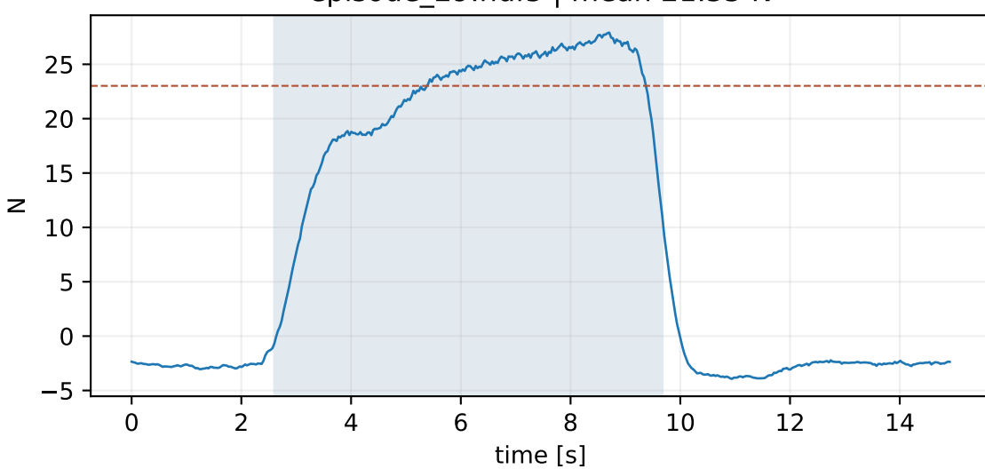
episode_29.hdf5 | mean 21.55 N
