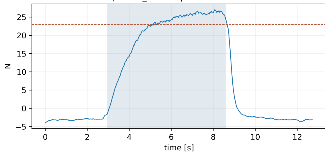
episode_3.hdf5 | mean 21.59 N
