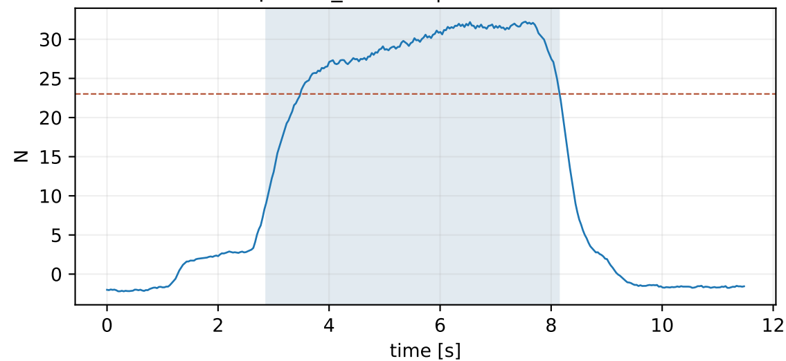
episode_34.hdf5 | mean 27.67 N
