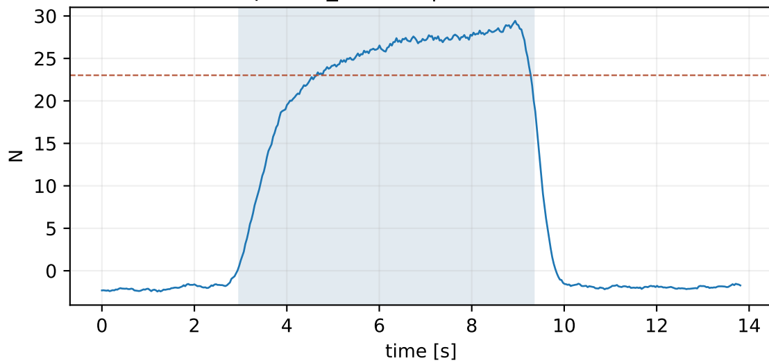
episode_36.hdf5 | mean 24.99 N
