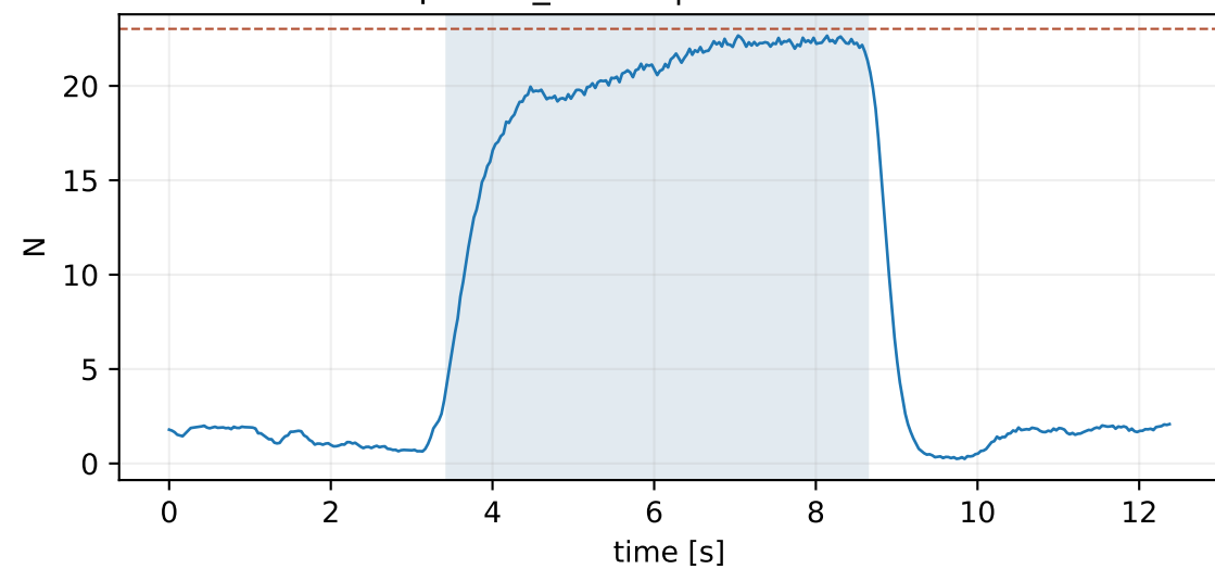
episode_5.hdf5 | mean 19.91 N
