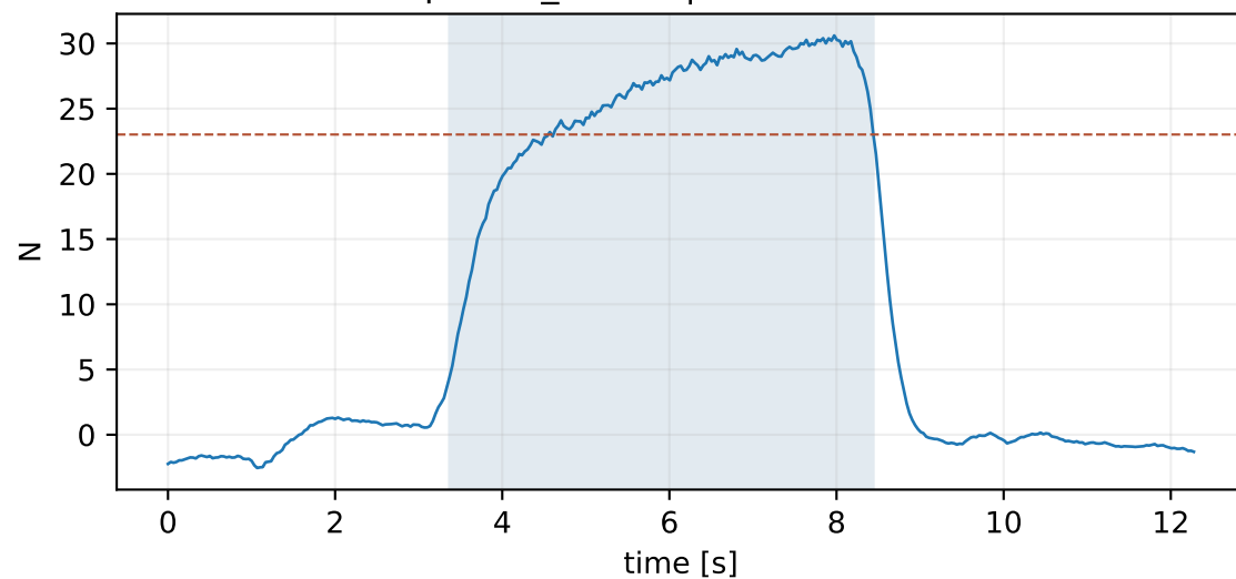
episode_11.hdf5 | mean 21.43 N
