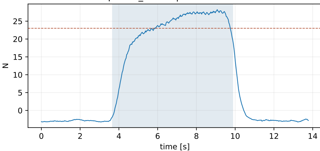
episode_8.hdf5 | mean 21.54 N
