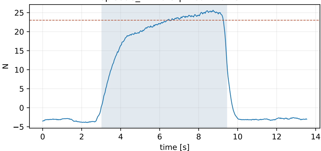
episode_14.hdf5 | mean 22.01 N
