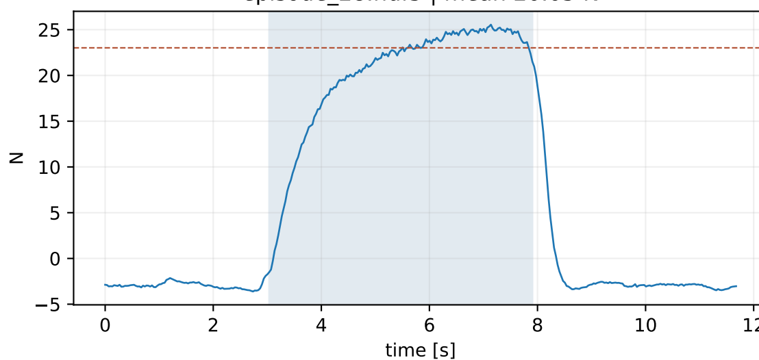
episode_30.hdf5 | mean 19.19 N
