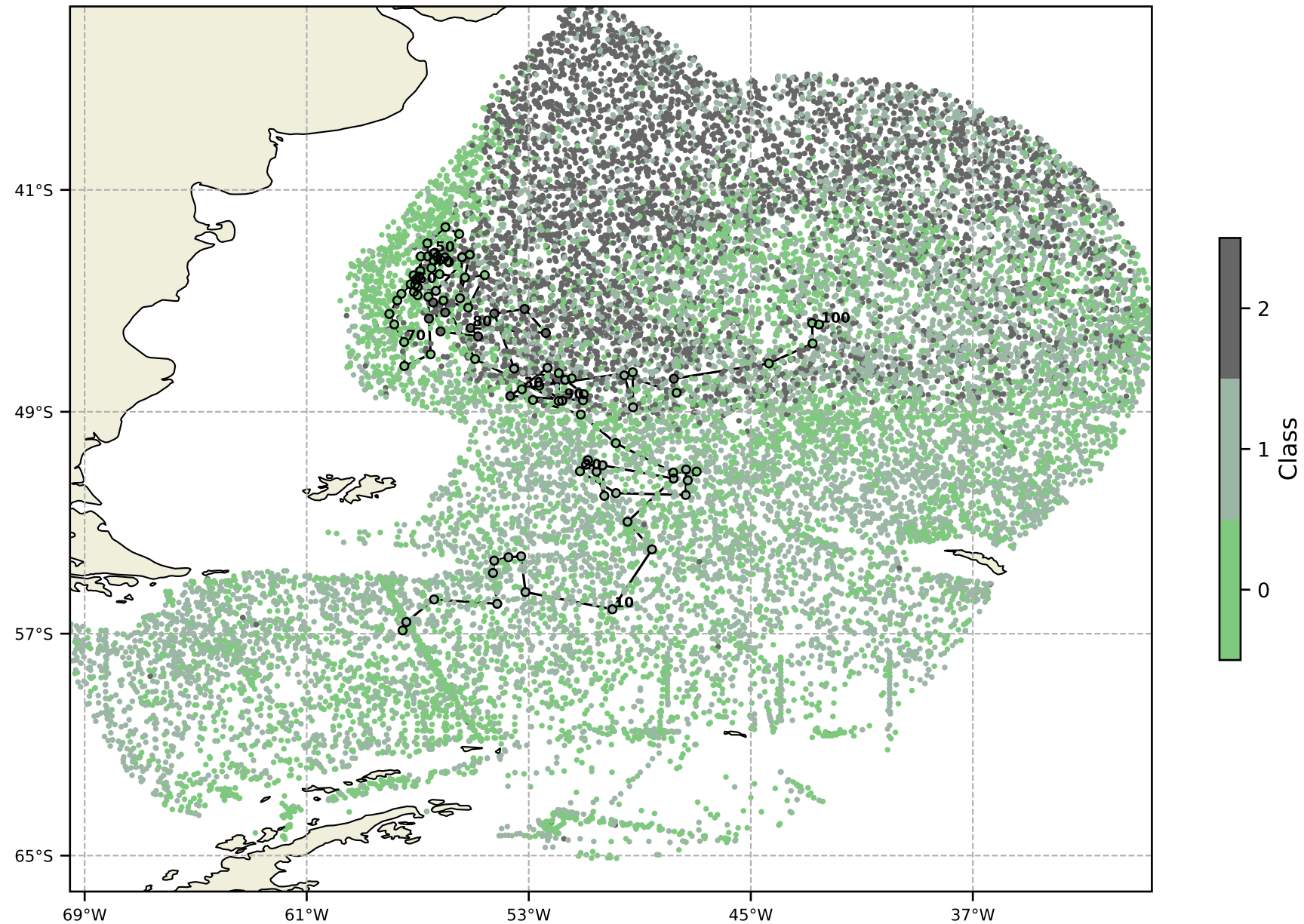
Spatial distribuion of classes (CTD database) for: 3900070
